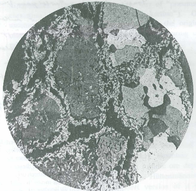
Fig. 1 Parties of rocks next the ore of Silberberg (Bodenmais) are traversed with loadings of zinc spinel (Kreittonit). Enlarging scale: 1:35, crossed nicols. From: Weinschenk 1901
