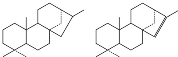
Fig. 8: Two examples for the phyllocladane carbon skeleton: \alpha -phyllocladane (left) and isophyllocladane (right).
