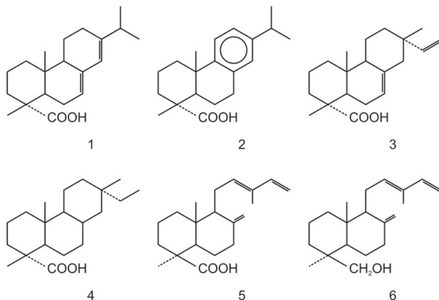
Fig. 2: Examples for diterpenoid resin acids and commanol: (1) abietic acid, (2) dehydroabietic acid, (3) isopimaric acid, (4) sandaracopimaric acid, (5) communic acid, (6) commanol.
