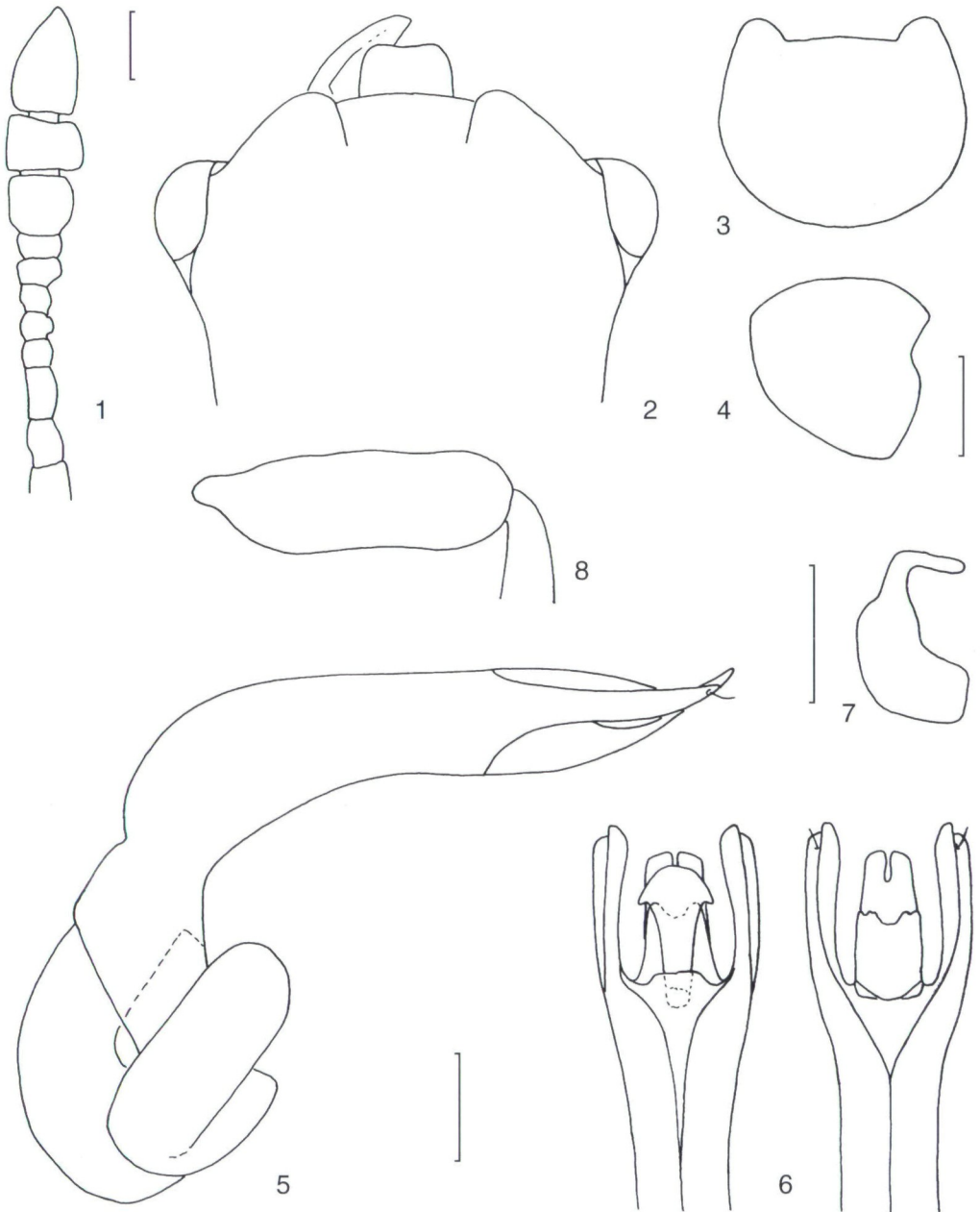
Figs. 1 - 8: Agathidium ( Microceble ) schillhammeri sp.n.: (1) antenna, (2) head, (3 - 4) pronotum in (3) dorsal and (4) lateral view, (5 - 6) aedeagus in (5) lateral, (6) ventral and dorsal view of apex, (7) spermatheca, (8) male hind femora; scale bar represents 0.1 mm (Figs. 1 - 2, 5 - 8), or 0.5 mm (Figs. 3 - 4).
