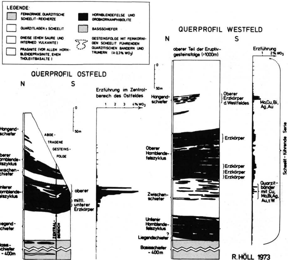
Fig. 16: Generalized stratigraphy of the Felbertal Scheelite Mine. After HÖLL, 1973.
