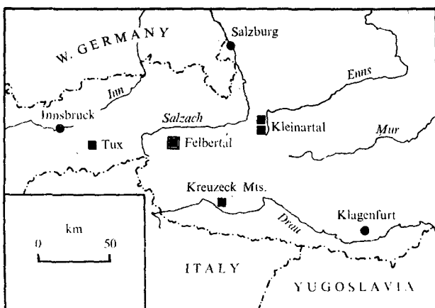
Fig. 12: Major scheelite occurrences in Austria (from STUMPF, 1977). Felbertal (Mittersill) is, at present, the only producing mine.
