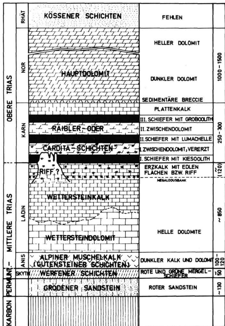
Fig. 9: Stratigraphy of the Triassic in the Bleiberg area (from M. BOUVIER et al., 1972). Crossed hammers indicate mineralized zones.
