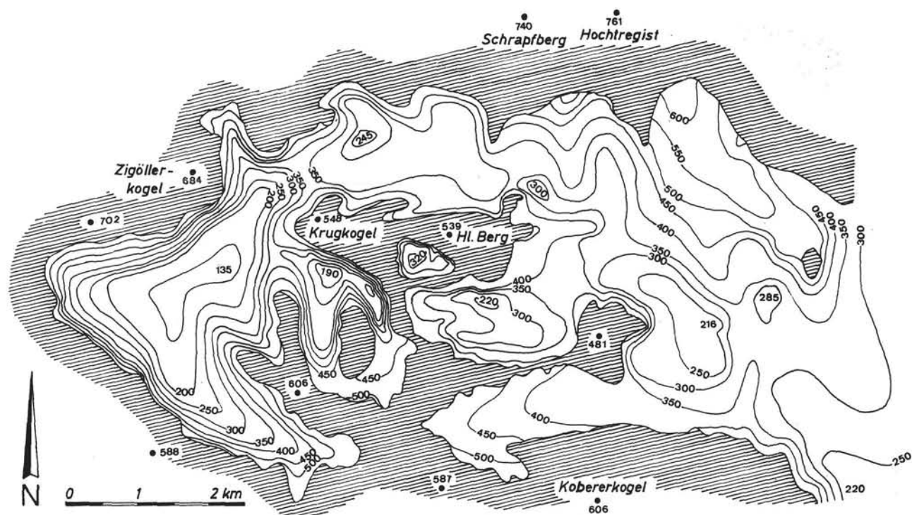
Fig. 2: Map of the pre-Tertiary relief of the lignite basin of Köflach—Voitsberg. After W. POHL, 1976.
