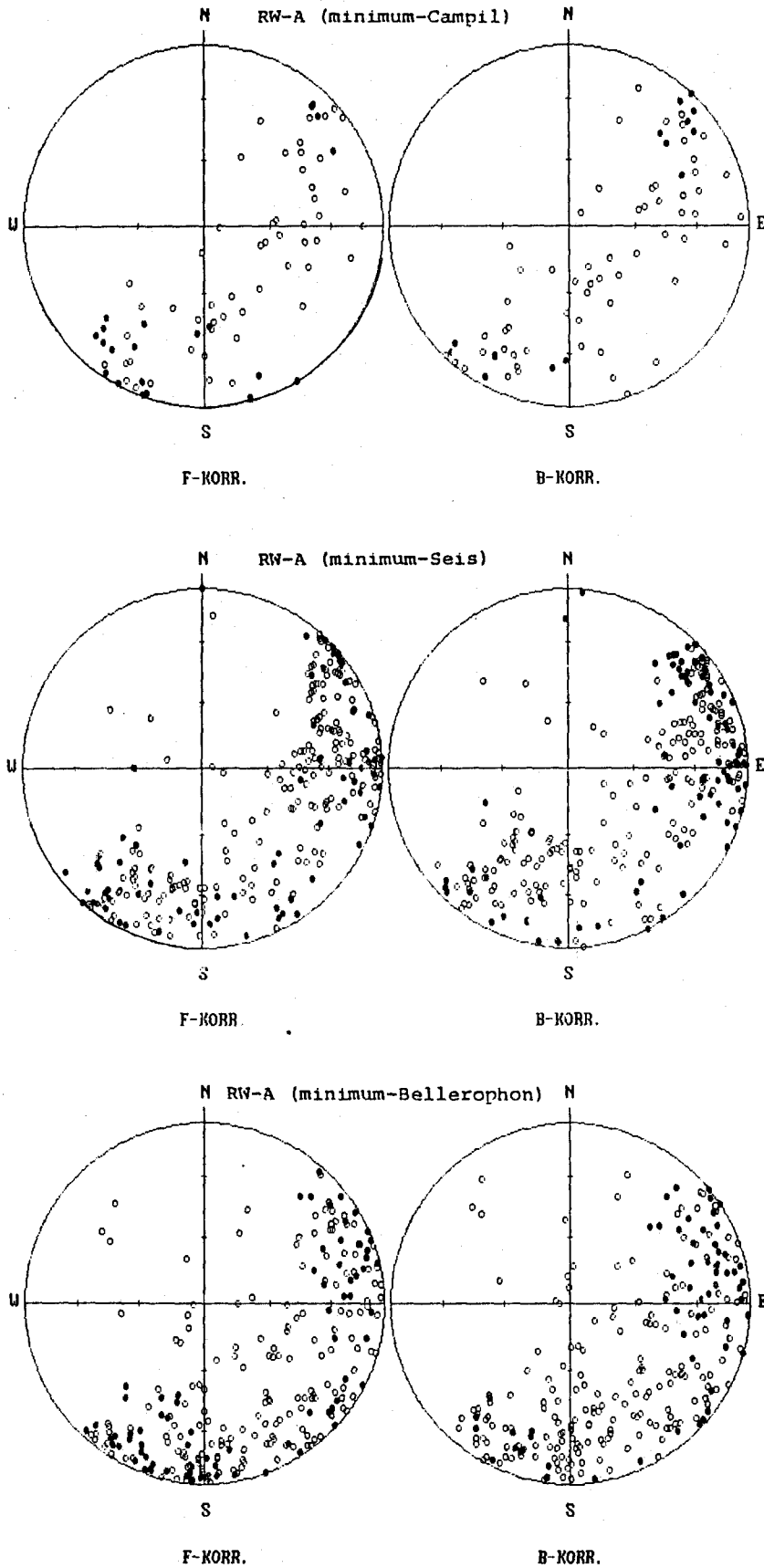
Text-Fig. 11. Demonstration of the scatter of the \kappa_{min} axes in each part of the section GK-1. Open symbols = inverse, closed symbols = normal.
