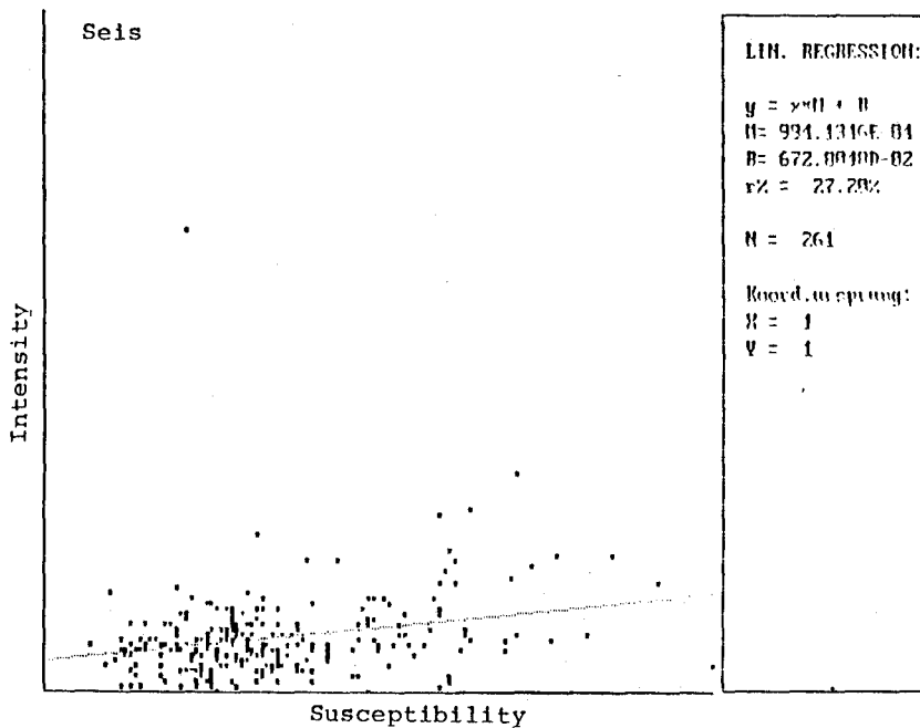
Fig. 6. Crossplots between susceptibility (x) and intensity (I) of all formations of the Gartnerkofel core GK-1: a) Campil. b) Seis. c) Bellerophon.
