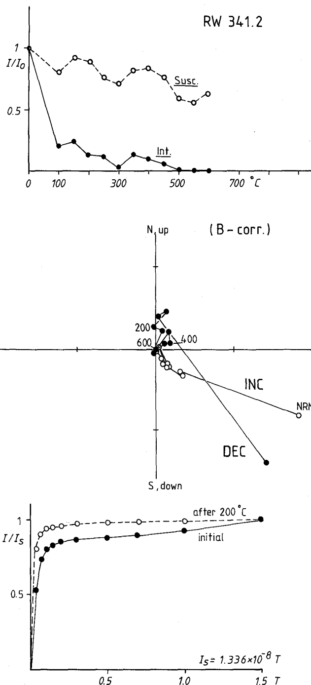
Text-Fig. 3. Example of rock magnetic data from the Bellerophon Formation, GK-1.
