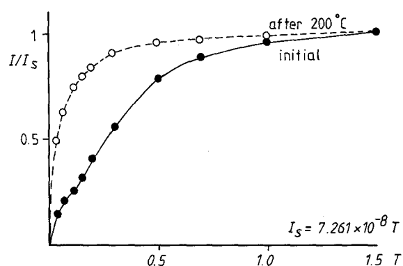
Text-Fig. 5. Example of rock magnetic data from the Werfen Formation (Seis Member), GK-1.
