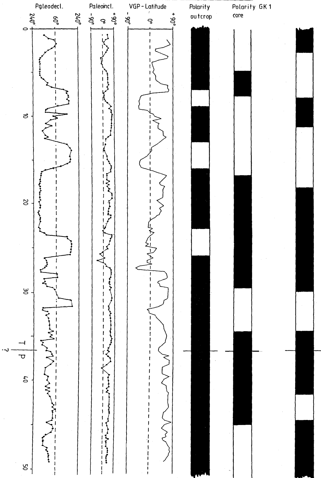
Text-Fig. 13. Magnetostratigraphic profile of the Reppwand outcrop section, compared with the corresponding section in the GK-1 core. Black = normal polarity; white = inverse polarity.
