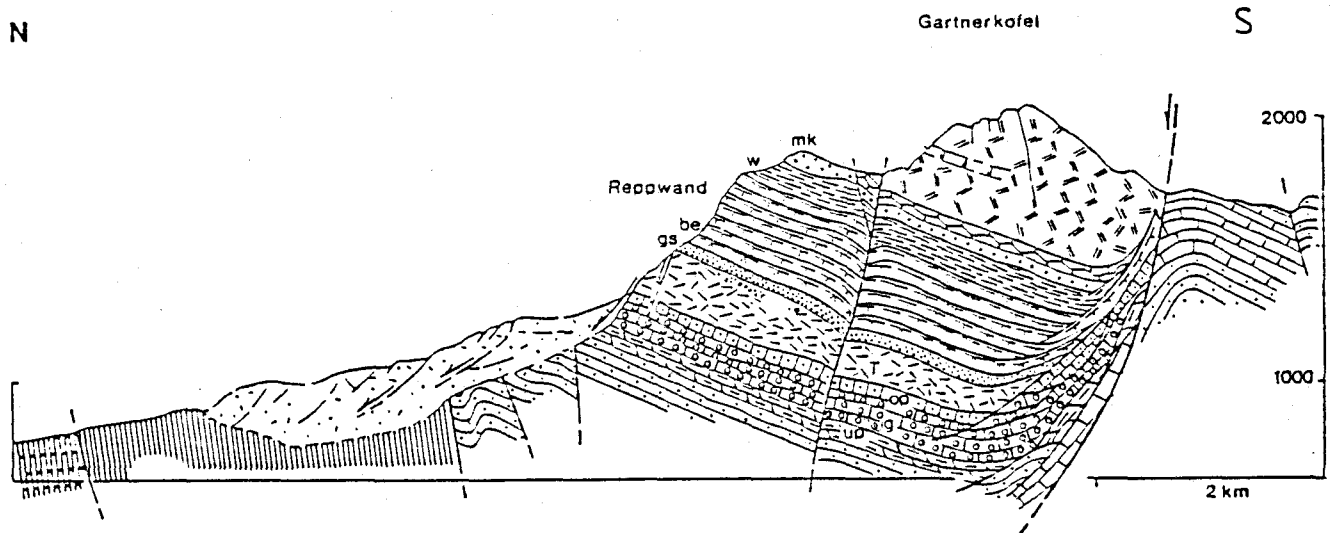
Text-Fig. 2. Geological profile of the Reppwand/Gartnerkofel area (F. KÄHLER & S. PREY, 1963).
