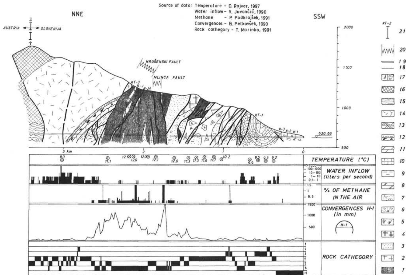
Text-Fig. 3. Geological cross-section of the Karavanke road tunnel – Slovenian part: Upper Carboniferous – Lower Permian clastic rocks with limestone lenses: 1 – Black schistose shale, 2 – Dark grey to black massive sandstone; Trogkofel limestone: 4 – Reddish and grey massive limestone; Trbiž/Tarvis breccia: 5 – Red limestone breccia; Gröden formation: 6 – Grey sandstone, conglomerate and breccia, 7 – Red schistose shale, siltstone, sandstone and conglomerate; Bellerophon formation: 8 – Grey, thick bedded dolomite, at places gypsum bearing; Werfen formation: 9 – Red to green micaceous dolomite and marl, gypsum bearing, 10 – Grey to reddish oolitic limestone, thin bedded; Anisian Dolomite: 11 – Grey to brownish medium bedded dolomite; Ukve/Uggowitz breccia: 12 – Variegated and grey carbonate breccia; red, green and grey marl, siltstone and calcarenite; Schlern dolomite: 13 – Grey bedded dolomite with chert, 14 – Light grey massive sparry dolomite; Rabelj/Raibl terrigene beds: 15 – Dark grey bedded limestone, marly limestone and dolomite; Formations of Klek/Hahnkogel unit: 16 – Dark grey to black mudstone, marl, marly limestone, limestone, dolomite, dolomite with chert, limestone with chert, mass flow breccia – not differentiated succession from Bača dolomite to Klek/Hahnkogel formation (after LEIN et al., 1995); Quaternary: 17 – Slope debris, moraine, 18 – Normal geological boundary, 19 – Fault plane, 20 – Fault zone, 21 – Surface borehole.
