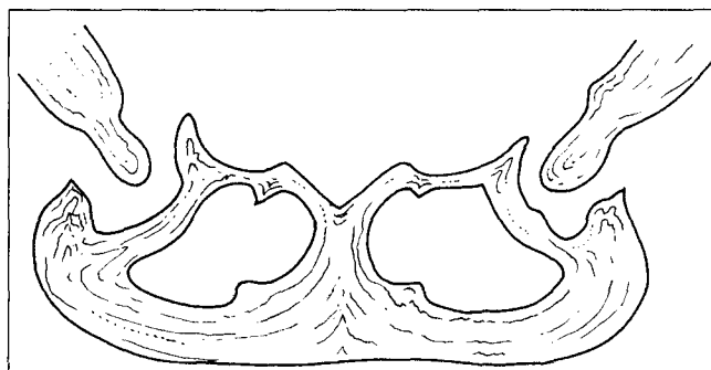
Text-Fig. 5. ? Cruratula sp. Transverse section through the posterior part of specimen showing well-developed hinge teeth, thick septalial plates and massive dorsal septum. GBA no. 1999/2/12. Magnified.
