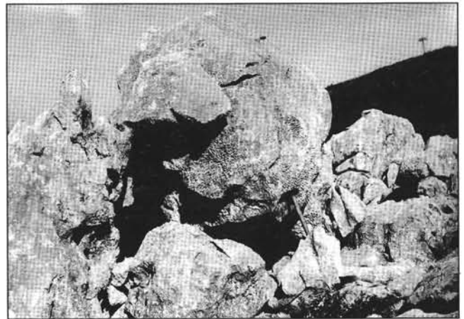
Text-Fig. 4. Retiophyllia buildup, Oberrhätalk-Capping Facies, "Fischer's Coral Garden".
