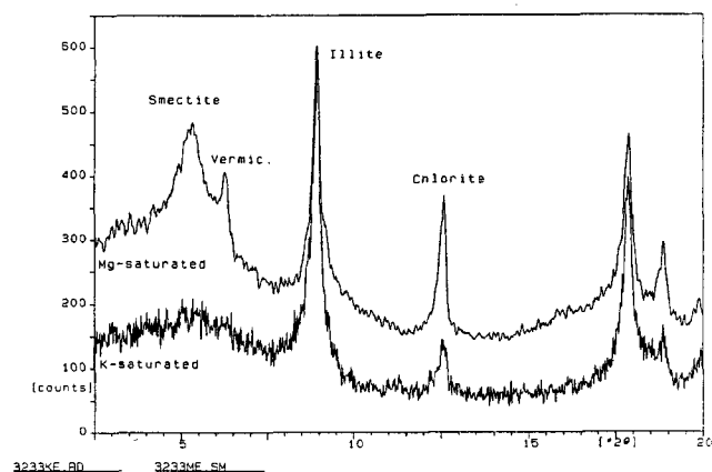
Text-Fig. 2. X-Ray-Diffractogram of sample GRÜ5, Late Campanian Inoceramus-Marls, <2\mu fraction, glycolated.
