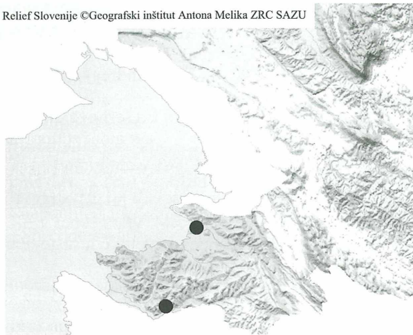
● Clivina ypsilon
