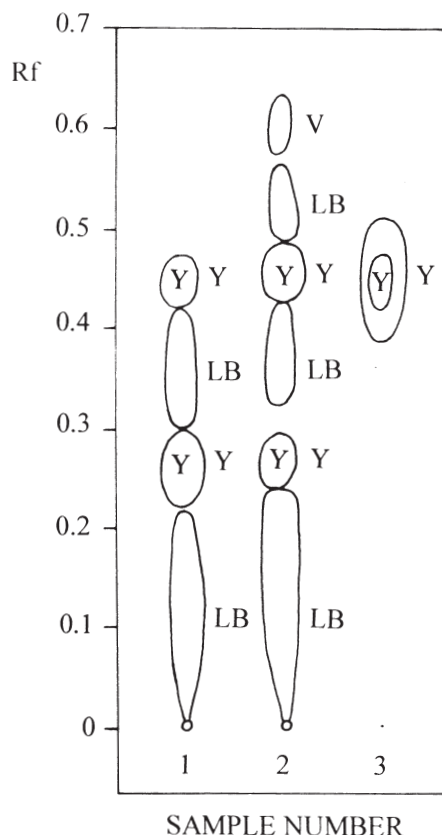
Fig. 3: Paper chromatography of extracts from wings of Libelloides macaronius . Samples: 1 – from yellow parts, 2 – from black parts, 3 – pure sepiapterin. Yellow spots, visible at daily light, are indicated with Y in the centre of spot. On the right side is indicated the colour of fluorescence at 365 nm: LB – light blue, V – violet, Y – yellow.
