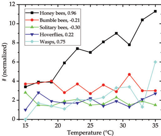
Fig. 6. Proportional number of pollinators in five categories depending on the outside temperature. Data at 15 °C and 35 °C correspond to all observations below and above the said temperature, respectively. Solid lines should be viewed as a guide to an eye. The value of Pearson correlation coefficient between the normalized number of pollinators and temperature is given in the figure legend for each category.
