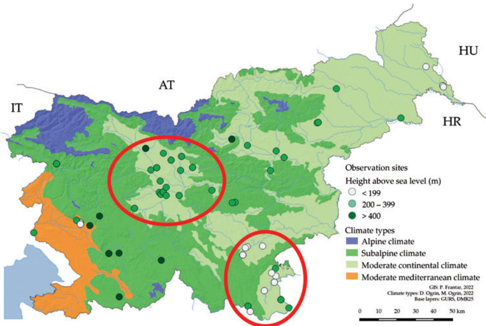
Fig. 1. Map of Slovenia representing observation sites according to their location (height above sea level and climate type). The two groupings of observation sites are indicated with red circles: one roughly covers Central Slovenia while another one is situated in Southeast Slovenia. Clusters based on the population density are not shown on the map.
