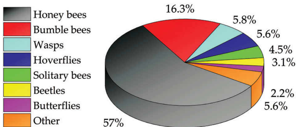
Fig. 2. A pie chart diagram representing the shares of individual categories of pollinator visits observed during the study.
