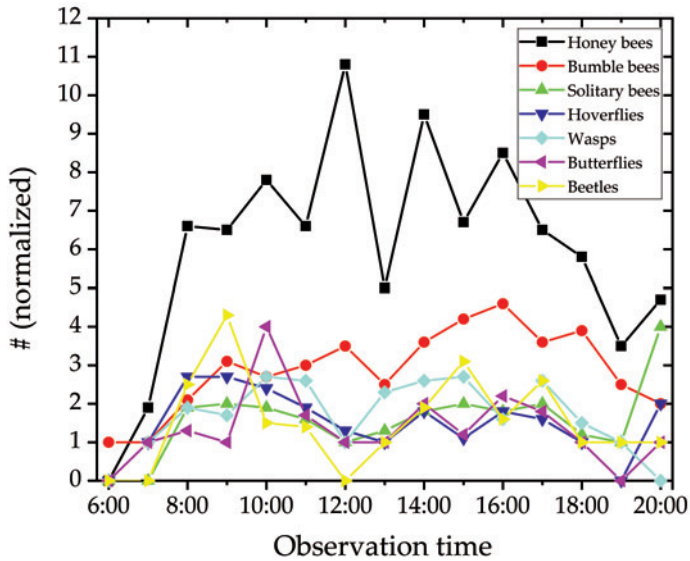
Fig. 5. Proportional number of pollinators by category depending on the part of the day. Solid lines should be viewed as a guide to an eye.
