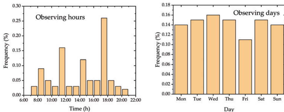
Fig. 4. Bar charts showing frequencies for observing hours (left) and days of the week (right).
