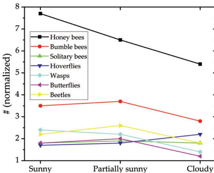
Fig. 7. Proportional number of pollinators by category depending on the type of the weather – reported for sunny, partially sunny, and cloudy. Solid lines should be viewed as a guide to an eye.
