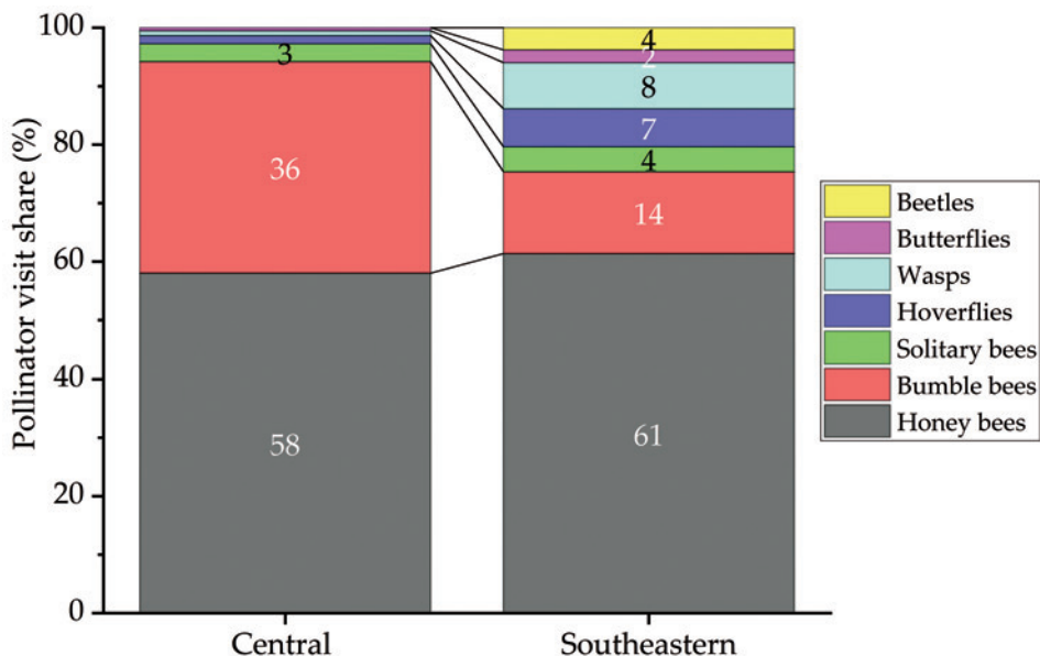
Fig. 10. Stacked column chart on pollinator communities for the two clusters. The total count of pollinators was 586 for Central and 3445 for Southeastern cluster.
