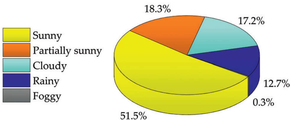
Fig. 3. A pie chart diagram representing the shares of different types of weather recorded during the study.
