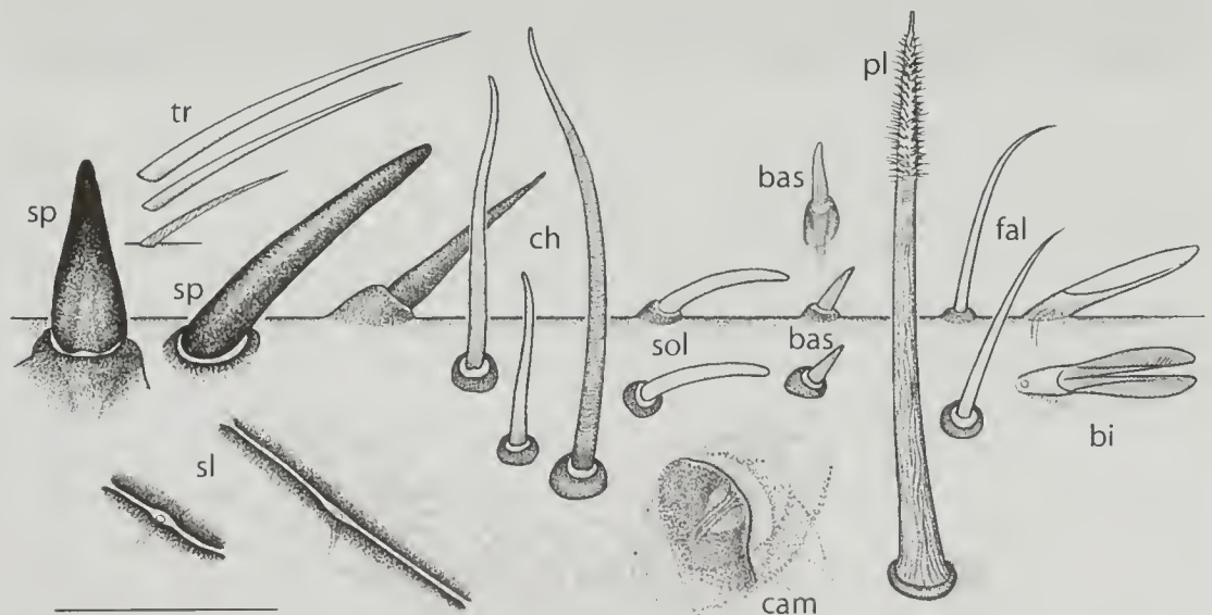
Fig. 2: Sensory structures and setae in D. ramosus with abbreviations used in figures (right is distal direction). From left to right: 2 spines (sp), 3 trichomes (tr), 2 slit sensilla (sl), 4 sensilla chaetica (ch), 2 solenidia (sol), 1 campaniform sensillum (cam), 3 sensilla basiconica (bas), 1 plumose seta (pl), 2 falciform setae (fal), 2 bipterate setae (bi). Scale bar: 50 µm.
