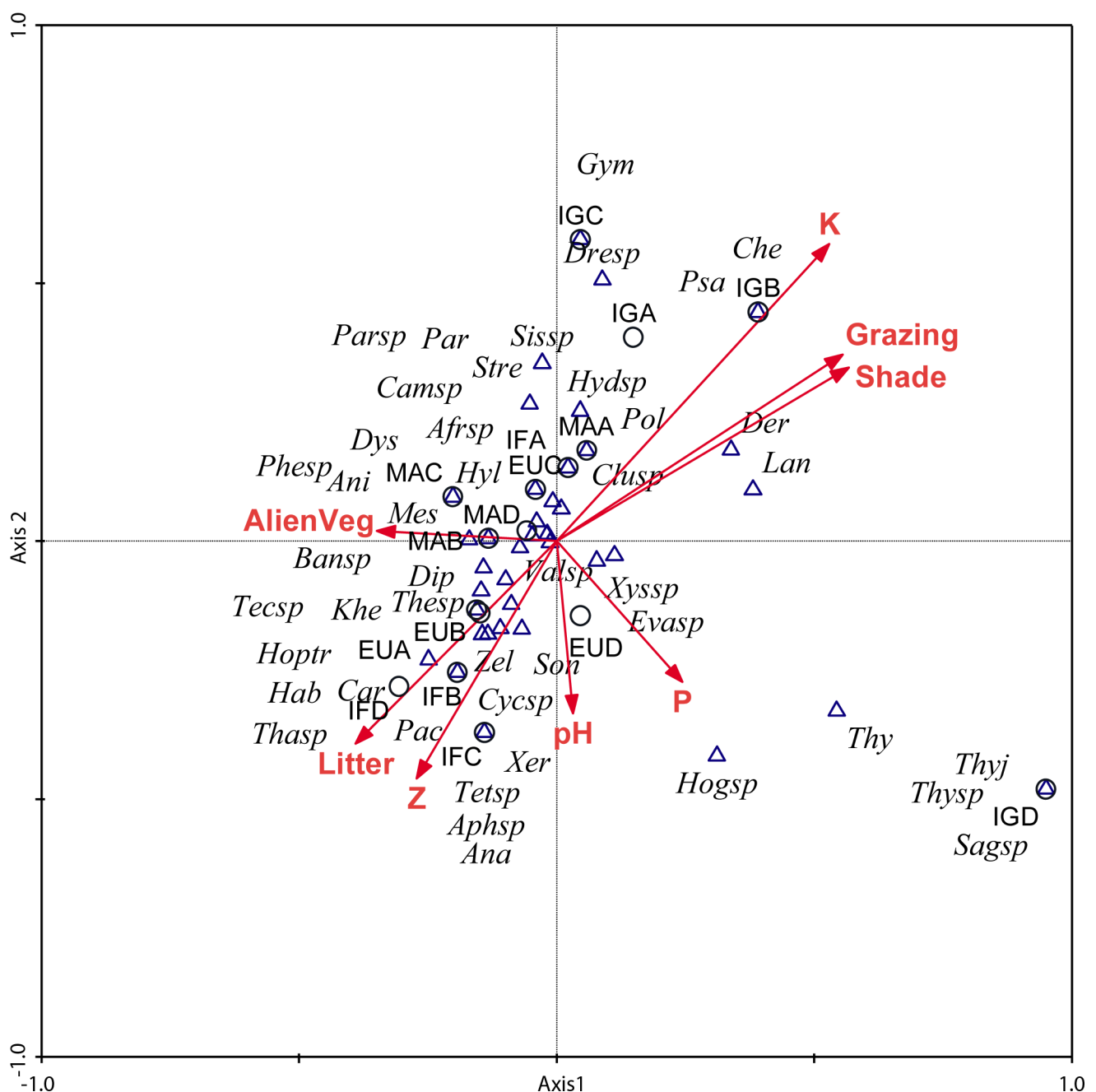
Fig. 2: Canonical Correspondence analysis (CCA) ordination of invertebrate species ( \Delta ), site sampling units ( \circ ), and measured environmental variables ( \rightarrow ) using pooled data collected at Nduli and Luchaba Nature Reserves. Site description and sampling unit labels see Tab. 1, species code names see Tab. 2.
