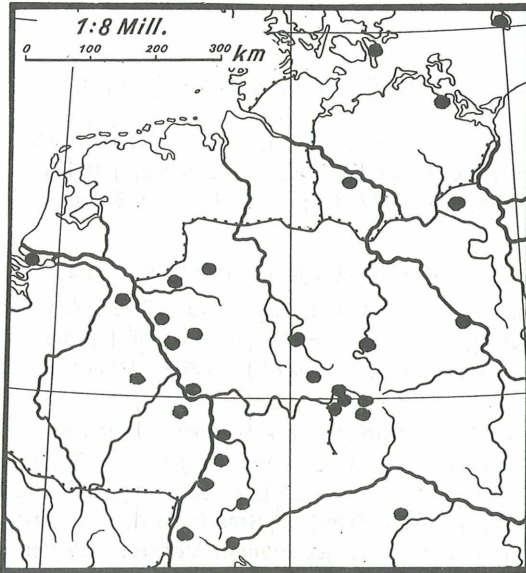
Abb. 5: Macdunnoughia confusa , Fundortkarte 1980
