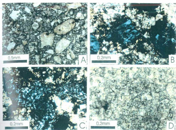
Figure 2: A – Devitrified and altered volcanic glass. B – Crystaloclast of feldspar. C – Chert (microcrystallised quartz). D – Rhomboedric crystals of dolomite.
