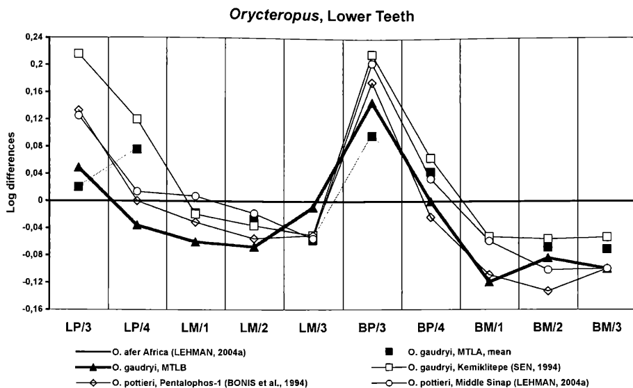
Figure 5: a. Logarithmic ratio diagram comparing the lower teeth of the Mytilinii material with Orycteropus gaudryi and Orycteropus pottieri . b. Logarithmic ratio diagram comparing the lower teeth of the Mytilinii material with various orycteropodids.
