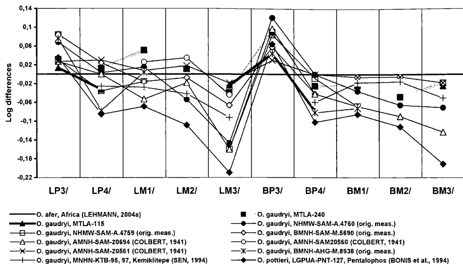
Figure 4: a. Logarithmic ratio diagram comparing the upper teeth of the Mytilinii material with Orycteropus gaudryi and Orycteropus pottieri . b. Logarithmic ratio diagram comparing the upper teeth of the Mytilinii material with various orycteropodids.
