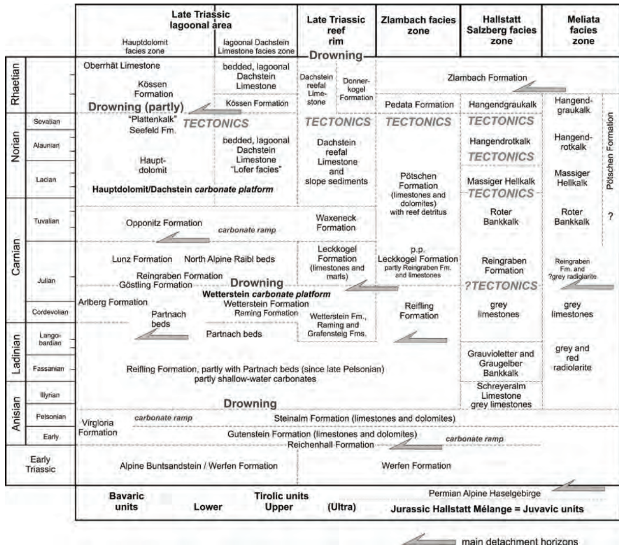
Figure 4: Lithostratigraphic table of Triassic formations and tectonic events in the central Northern Calcareous Alps (modified after TOLLMANN, 1985; GAWLICK & FRISCH, 2003; PILLER et al., 2004; MISSONI & GAWLICK, 2011a, b). The main detachment horizons are indicated because of their importance during Jurassic nappe stacking and disintegration of the sequence in the course of mélange formation. The colours of the different facies belts in this figure correspond to the colours in the other figures, clarifying the provenance of the different clasts and slides in the Jurassic basin successions (after MISSONI & GAWLICK, 2011a). Compare also Fig. 6.
