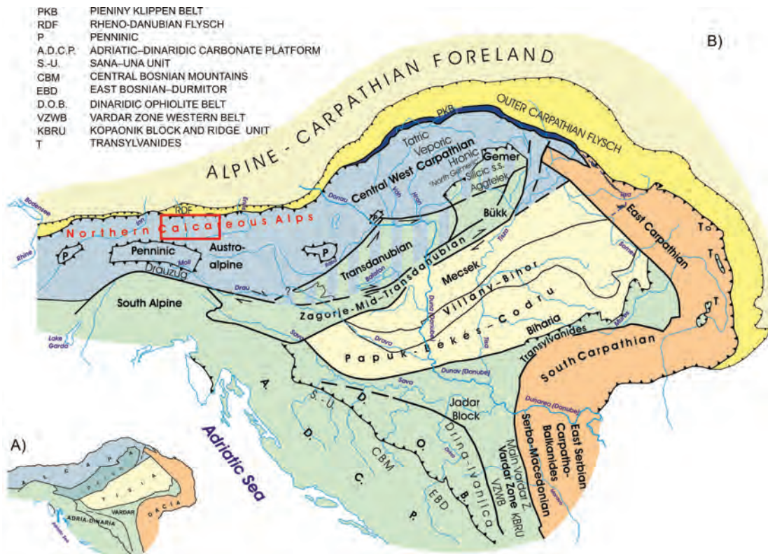
Figure 1: A) Mega-units and mountain belts in the Alpine-Carpathian-Dinaride-Pannonian realm. B) Most important tectonic mega-units/nappe systems in the Alpine-Carpathian-Dinaride-Pannonian realm with more detailed names of the different units and the area of the field trip indicated (after KOVACS et al., 2010, 2011). For the Austroalpine mega-unit and the exact geographic position of the Northern Calcareous Alps see Fig. 2.
