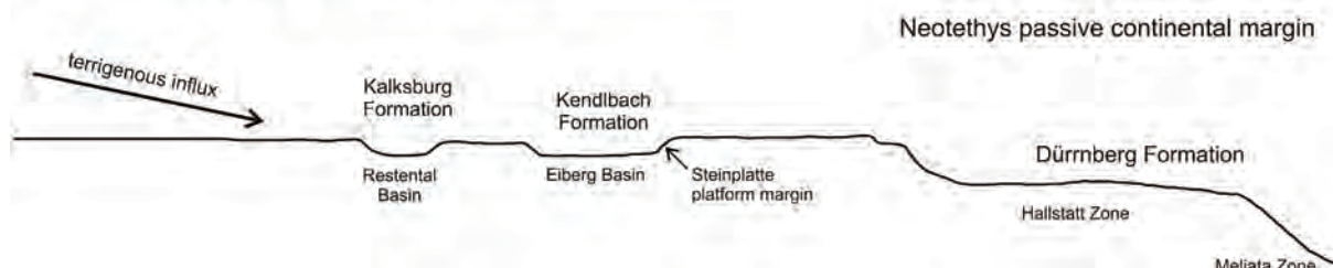
Figure 13: Two profiles showing the palaeotopographic situation in the Austroalpine domain. A) Sedimentation in the earliest Jurassic was controlled by the end-Triassic morphology of the exposed or drowned Hauptdolomit/Dachstein Carbonate Platform s. l. with the Eiberg Basin in a central position (e.g., GOLEBIEWSKI, 1991; KUERSCHNER et al., 2007; BONIS et al., 2009) and the Restental Basin (= later Allgäu Basin; GOLEBIEWSKI, 1990b) in a more continent-ward position. B) Later in the Early Jurassic (Late Hettangian) crustal extension in the Penninic realm controlled the basin formation, geometry and sedimentation. The Early Rhaetian Kössen beds below the Rhaetian Dachstein Limestone (south of the Eiberg Basin) and Oberrhät Limestone (north of the Eiberg Basin) could have formed the detachment horizon (line in upper profile), on which Penninic crustal extension affected also the Tirolic realm of the Northern Calcareous Alps in the Late Hettangian/Early Sinemurian. Breccia formation on the Penninic passive continental margin lasted from Late Hettangian to Early Pliensbachian times.
