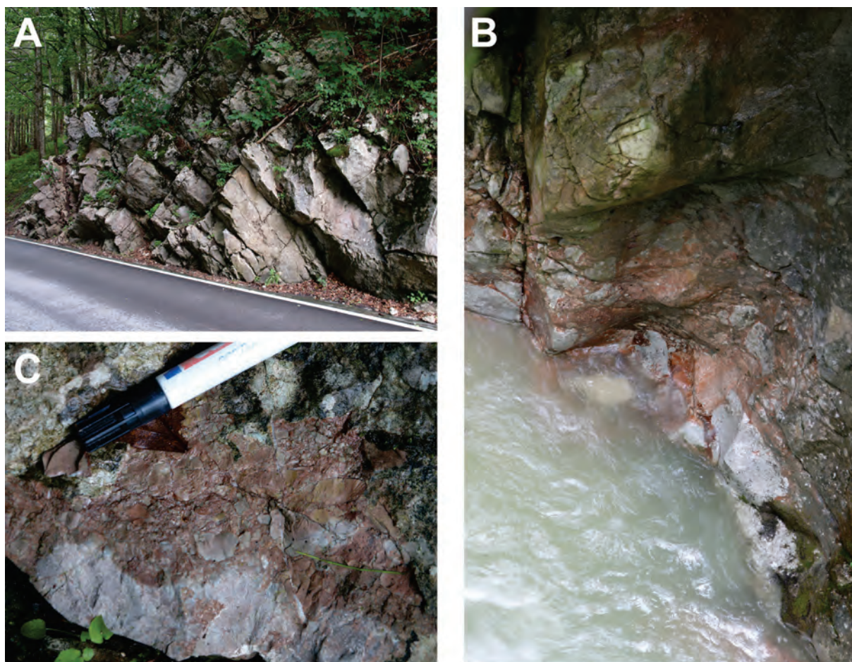
Figure 26: Sandlingalm Formation in the Zauberwald area.
