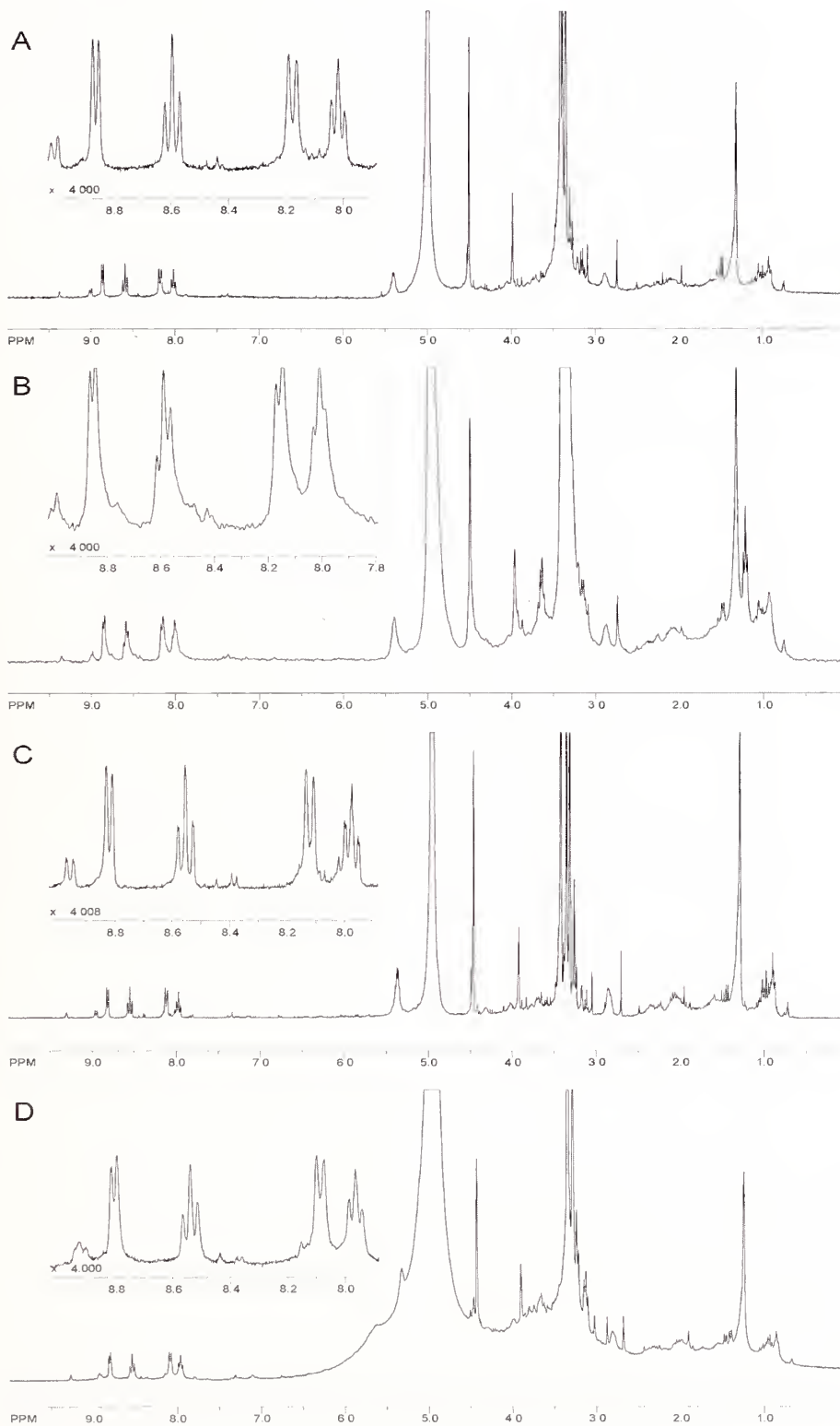
Fig. 3. ^1\text{H} NMR spectra of crude extracts of dissected Mariona blainvillea in methanol- d_4 , 300 MHz. A. Mantle, B. Foot, C. Digestive gland, D. Viscera without digestive gland.
