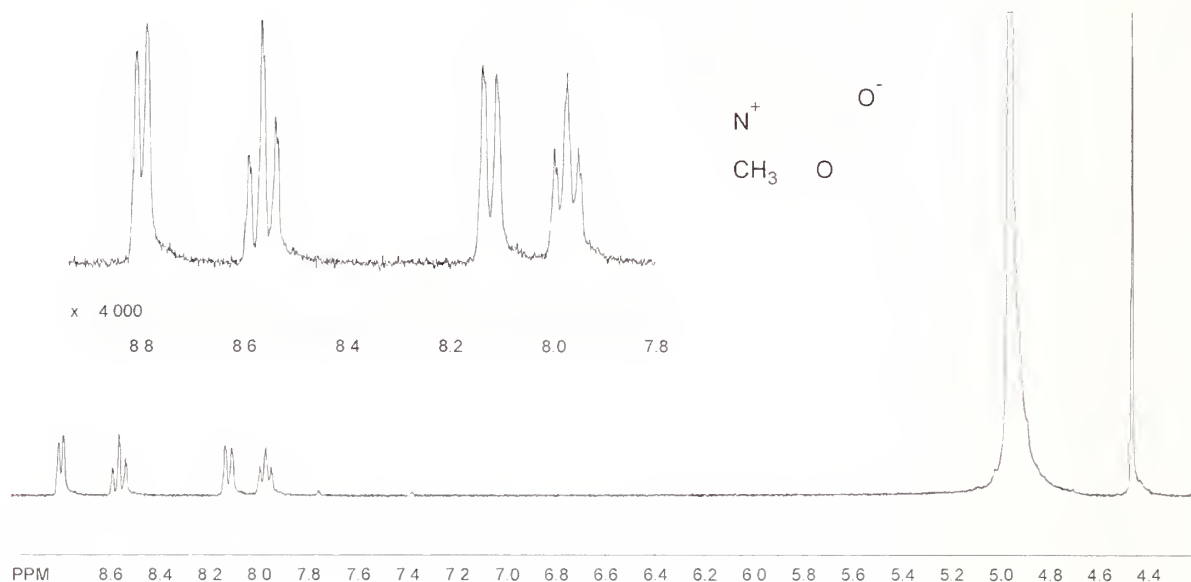
Fig. 2. ^1\text{H} NMR spectrum of purified homarine in methanol- \text{d}_4 , 300 MHz, and chemical structure of homarine.
