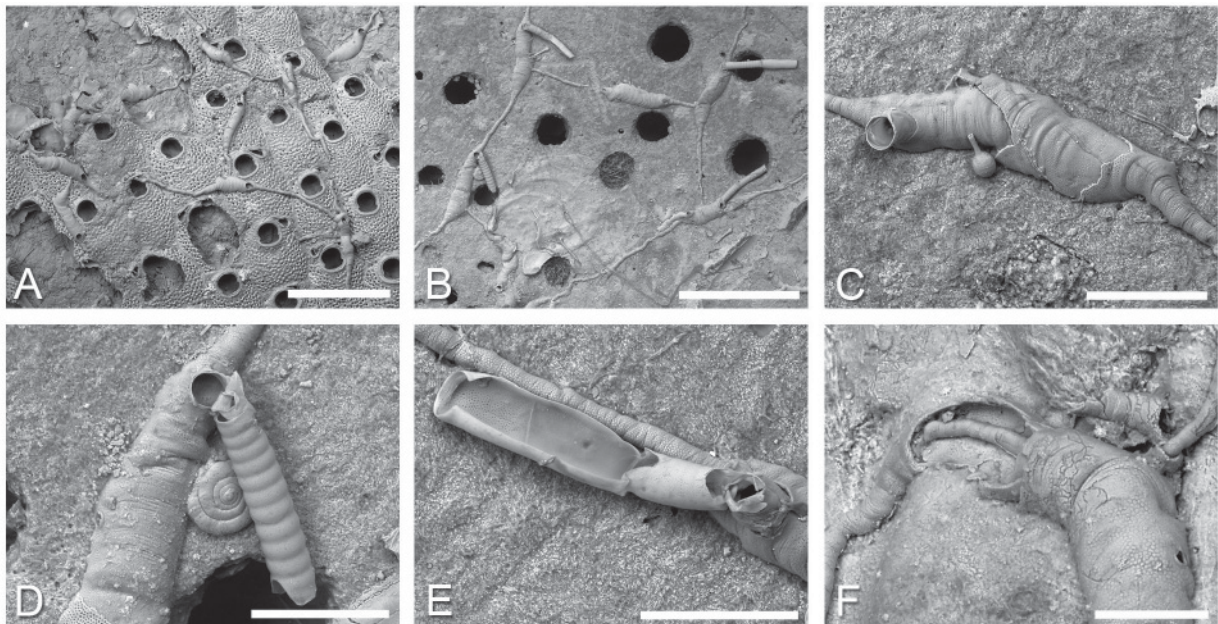
Fig. 2. Aetea ligulata Busk, 1852. A. Colony fouling Hippopodina feegeensis ; Pantai Pasir Hitam, Langkawi, MSL BRY001a. B–F. Kampung Kuala Temoyong, Langkawi, MSL BRY002. B. Zooids growing around clionid-bored shell. C. Zooid with repaired skeleton. D. Erect part of zooid collapsed against substrate to reveal annulations on distal side. E. Erect part of zooid collapsed to show opesia on proximally facing side. F. Broken zooid showing intramural ‘stolon’. Scale bars: A–B = 1 mm; C–E = 200 µm; F = 100 µm.
