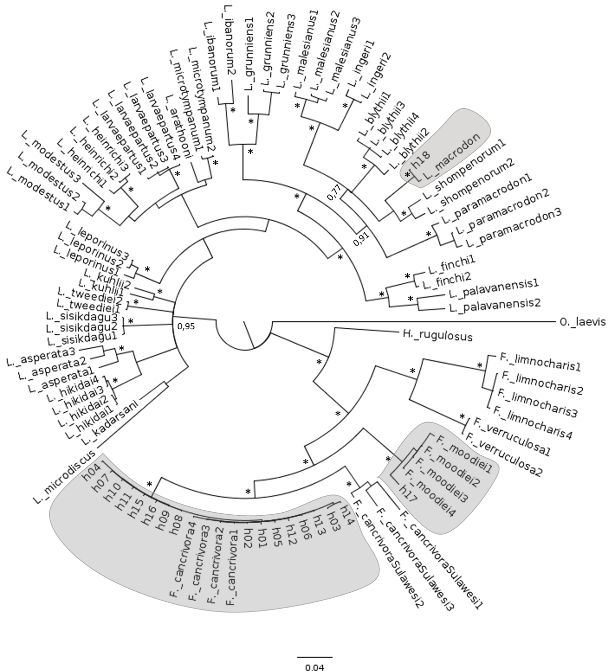
Fig. 1. Phylogeny of Indonesian species of Fejervarya and Limnonectes recovered by the Bayesian analysis (GTR+I+G model). Hoplobatrachus rugulosus (Wiegmann, 1834) and Occidozygia laevis (Günther, 1858) were used as outgroups. Numbers on nodes represent Bayesian posterior probabilities, * indicates a value higher than 0.98. Only values higher than 0.75 are represented. h01 to h18 indicate the 18 haplotypes from frozen frog legs recovered in this study.
