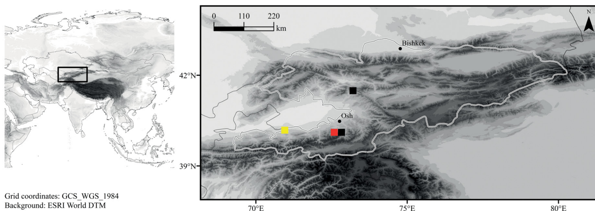
Fig. 1. Relief map of part of Asia with detail of Kyrgyzstan and adjacent regions with the localities at which dipturans were found; Kyrgyzstancampa sanare Sendra & Ferreira gen. et sp. nov. (yellow square); Campodea (Dicampa) catalana Denis, 1930 (red square); Turkmenocampa edaphica Sendra & Sánchez-García sp. nov. (black square).
