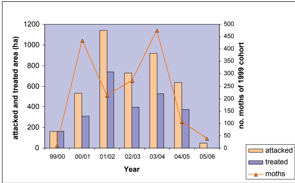
Fig.2: Attacked and treated area in Venosta/Vinschgau during 1999-2006, compared with the total number of moths emerged from 3 cages where colonies of the 1998-99 cohort were allowed to pupate.
