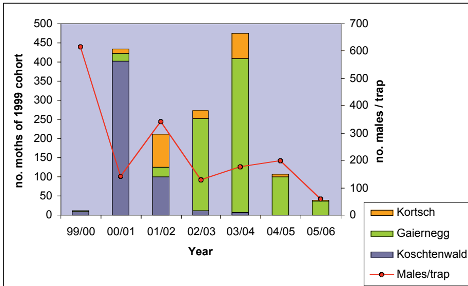
Fig.3: Emergence of the moths of the cohort 1998-99 (pupated in April 1999) inside the experimental cages at 3 sites on the southern slope of Venosta/Vinschgau, compared with the number of adult males caught in pheromone traps in the same area.
