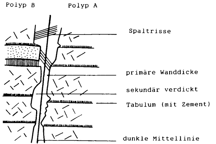
Favosites
