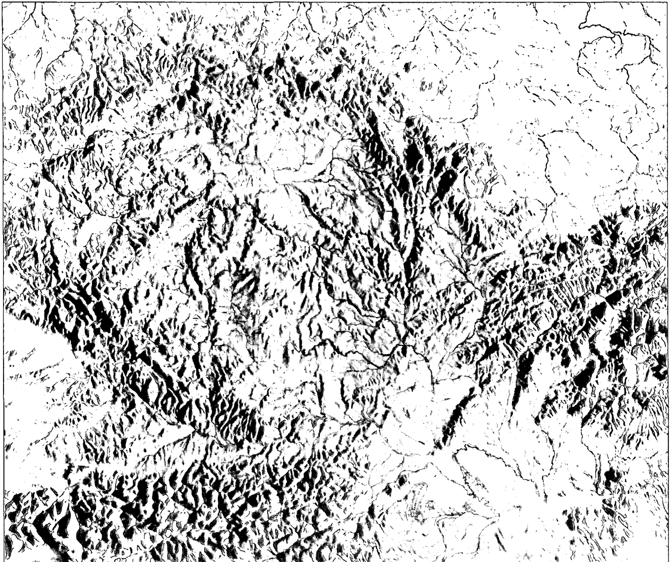
Text-Fig. 2. Relief map photograph of the Bohemian Massif illuminated from the East.
