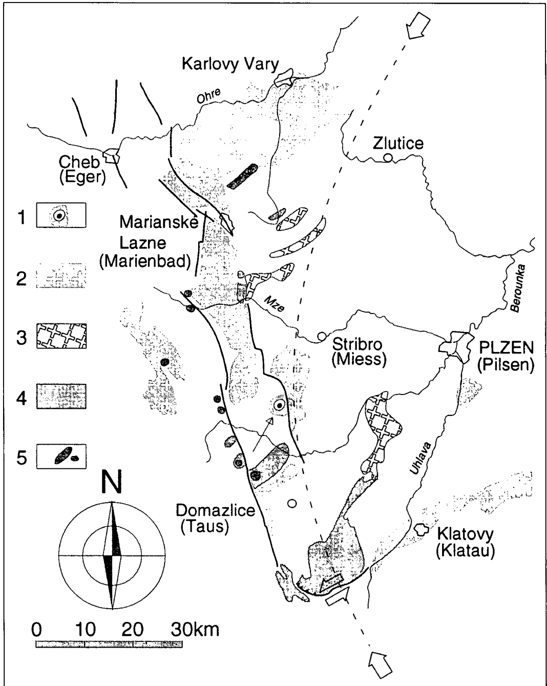
Text-Fig. 8. Example of the detailed correlation of geological data in Western Bohemia with the circular structure from the fit to the topographical lineaments. 1 = Sedmihori intrusive ring structure; 2 = Variscan granites; 3 = Panaf-rican granites; 4 = Panaf-rican gabbros; 5 = ultra-maphic rocks.
