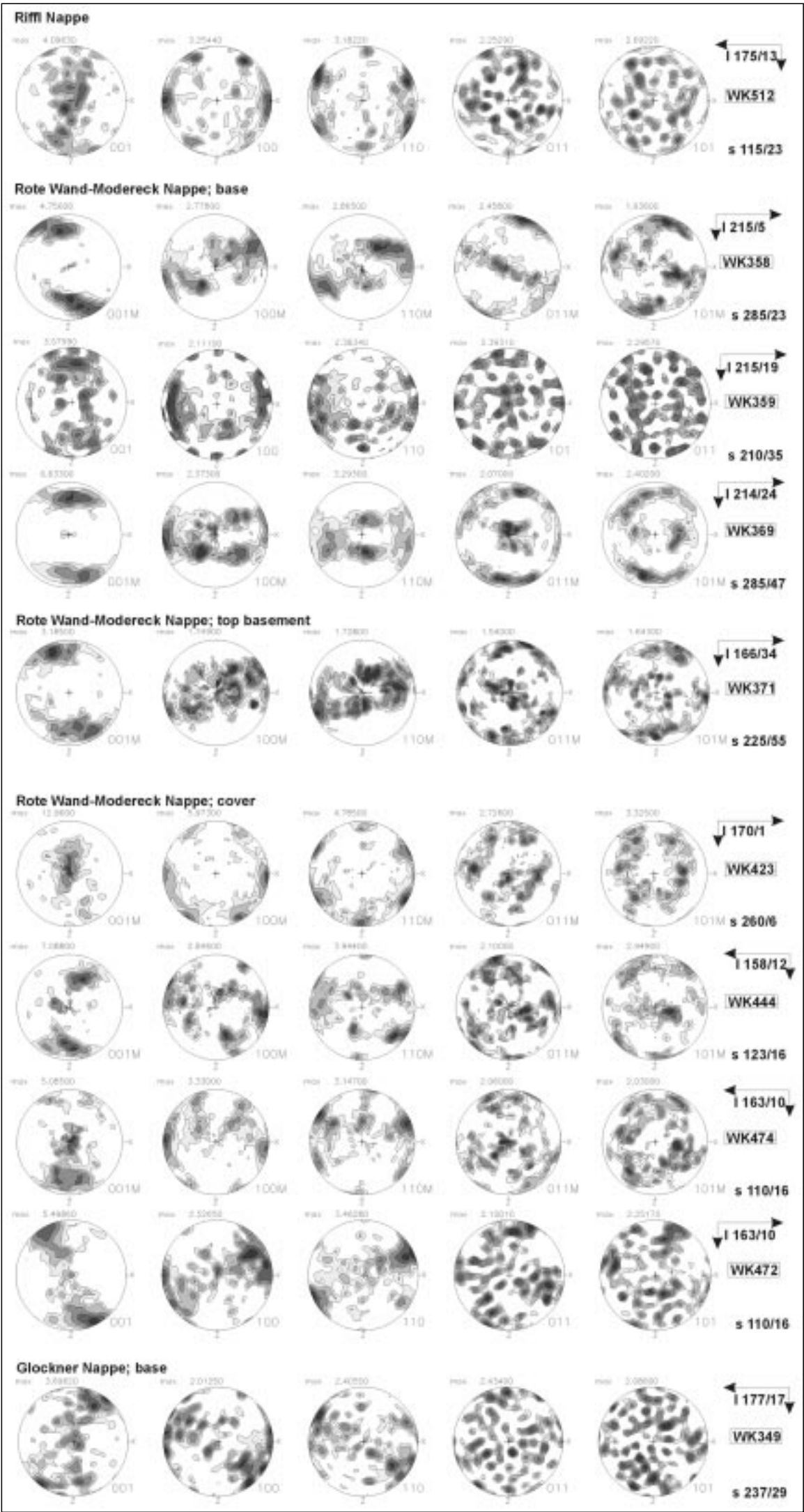
Text-Fig. 6. Representative quartz CPOs that are related to de- formation phase D 1 , central Tau- ern Window. Equal angle pro- jections; logarith- mic gradation of isolines. First isoline: uni- form distribution; fifth isoline: 85 % of maximum; M: calculation by us- ing the Vector method of SCHAE- BEN et al. (1985); SCHAEBEN (1994).
