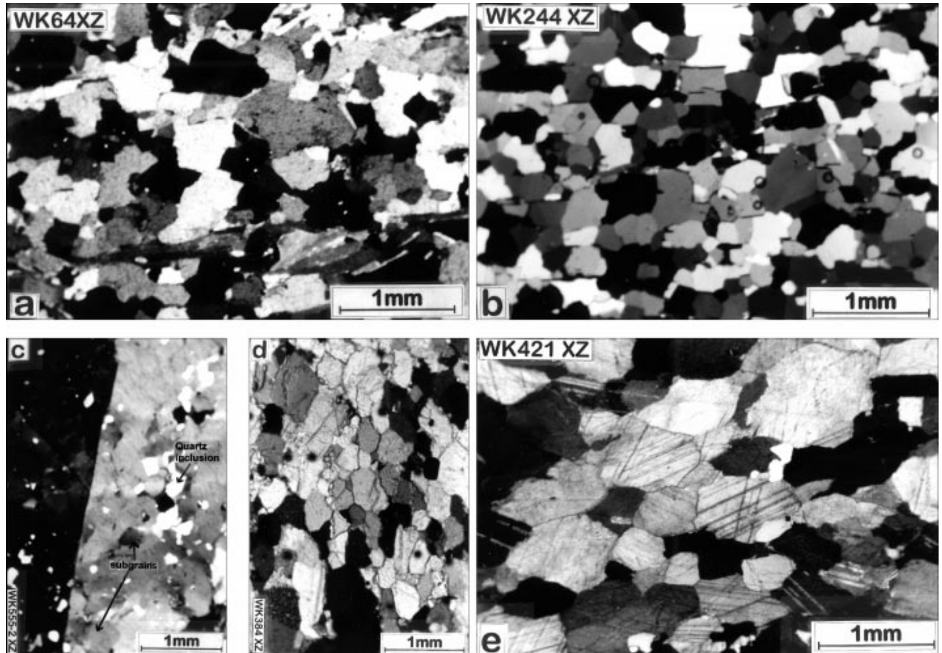
Text-Fig. 3. Representative microstructures that are related to deformation phase D 1 . a) Annealed quartz microstructure, Venediger Nappe, southeastern Tauern Window. b) Equilibrated quartz microstructure, Glockner Nappe, northeastern Tauern Window.
