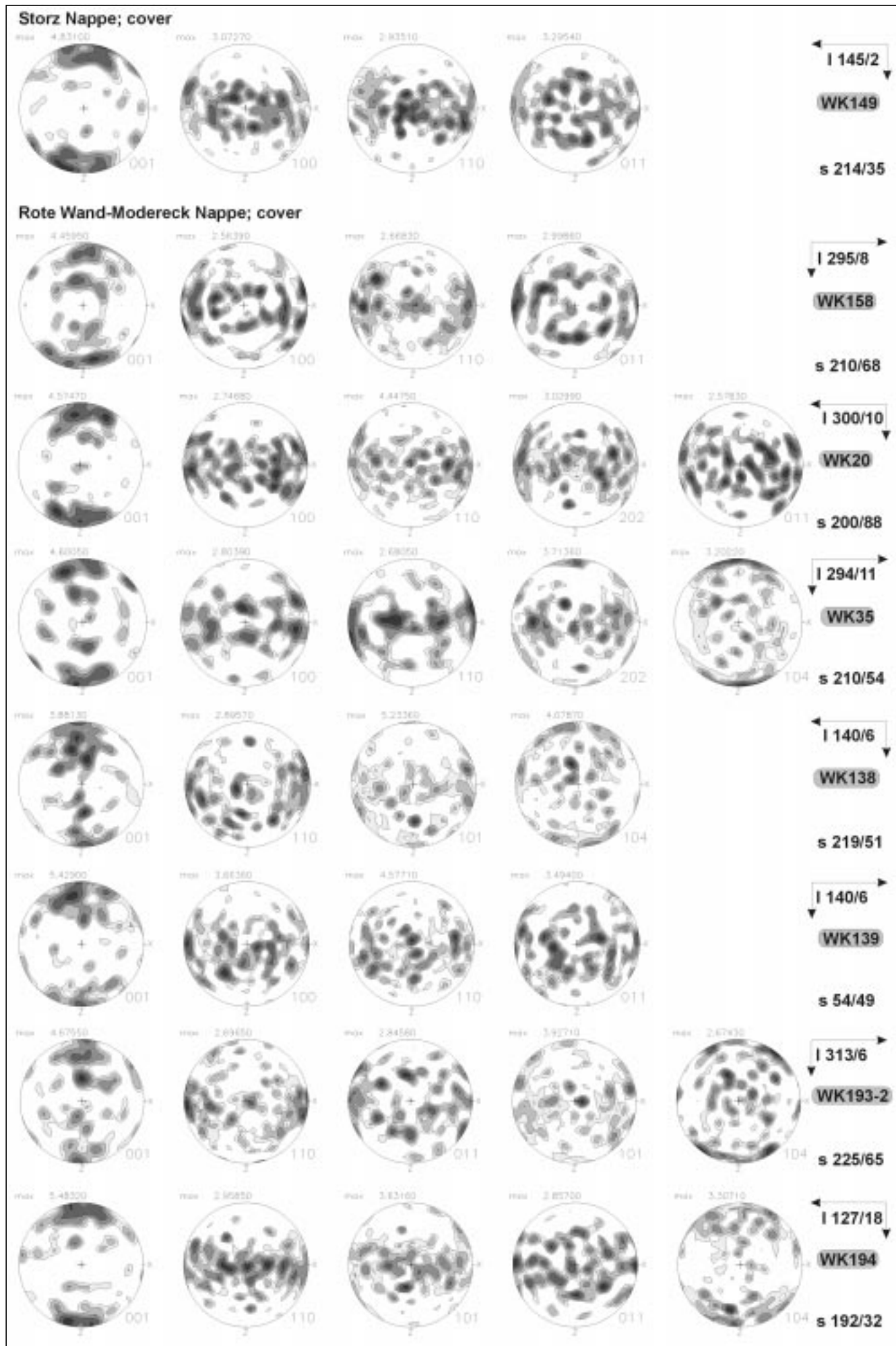
Text-Fig. 20. Representative calcite CPOs that are related to D_2 . Southeastern Tauern Window. For explanation see Text-Figs. 5, 6.
