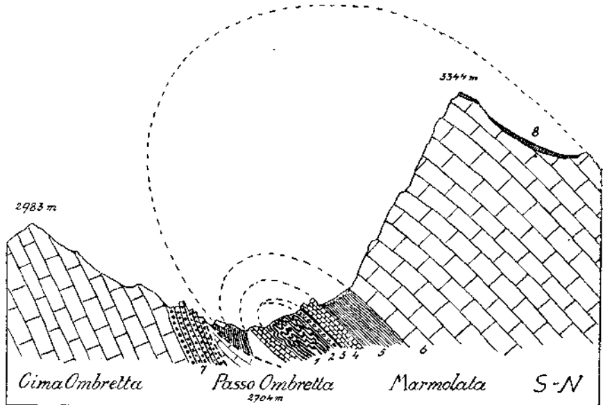
Fig. 4. 1 = Werfener Schichten. 2 = Riechhofenkonglomerat. 3 = Unterer Muschelkalk. 4 = Mendoladolomit. 5 = Buchensteiner Schichten. 6 = Marmolatakalk. 7 = Tuffkonglomerate. 8 = Gletscher.
