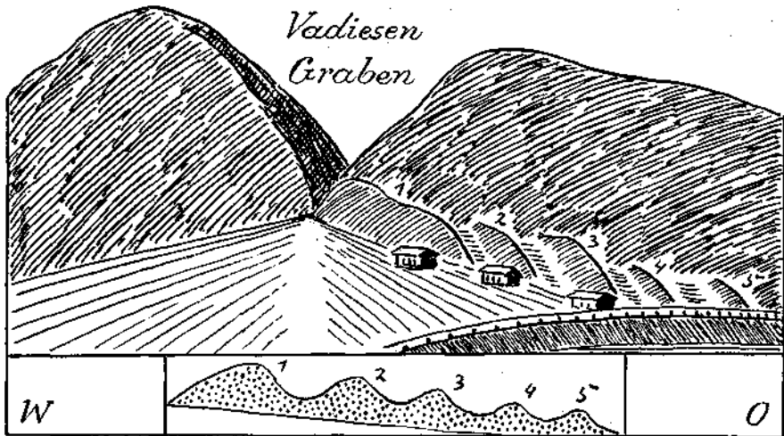
Fig. 13. 1, 2, 3, 4, 5 = Endmoränenwälle.
