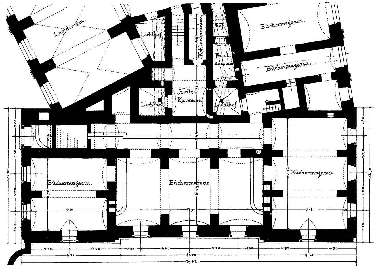
Sockelgeschoss.
