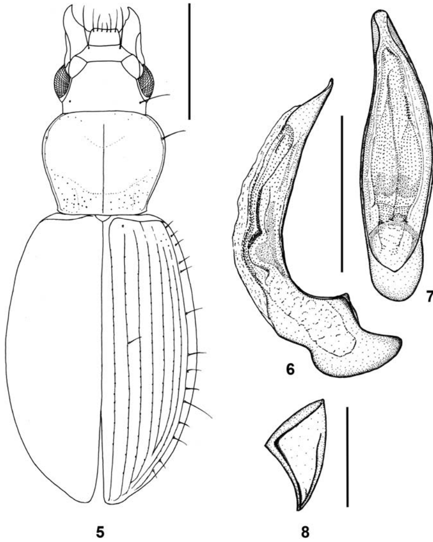
Figs 5-8: Psychristus (Nipponobradycellus) umbraticornis nov.sp. Habitus (5). Median lobe, lateral view (6), median lobe, dorsal view (7). Left metepisternum (8). Scale bars: 1 mm (5); 0.5 mm (6, 7, 8).
