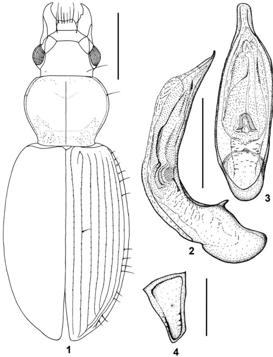
Figs 1-4: Psychristus (Nipponobradycellus) schmidti nov.sp. Habitus (1). Median lobe, lateral view (2), median lobe, dorsal view (3). Left metepisternum (4). Scale bars: 1 mm (1); 0.5 mm (2, 3, 4).
