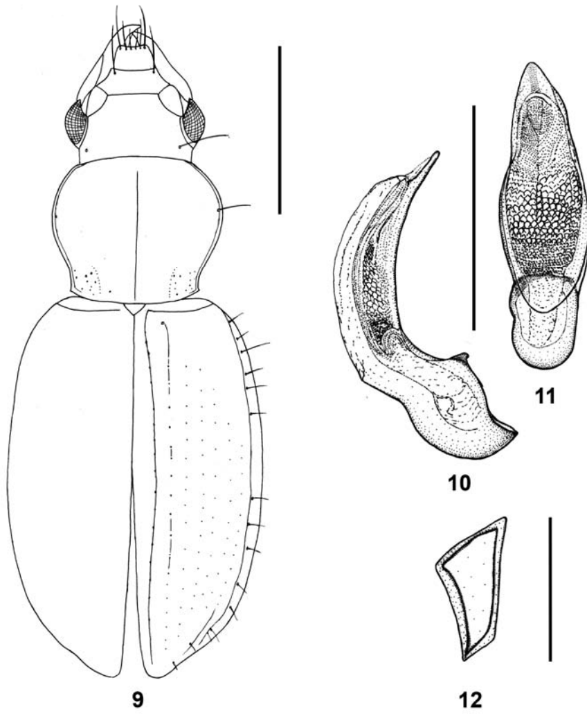
Figs 9-12: Psychristus (Nipponobradycellus) glaber nov.sp. Habitus (9). Median lobe, lateral view (10), median lobe, dorsal view (11). Left metepisternum (12). Scale bars: 1 mm (9); 0,5 mm (10, 11, 12).
