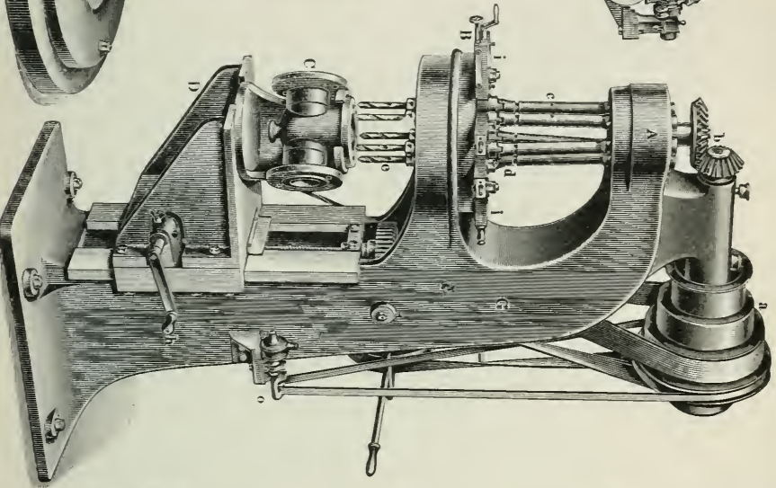
3. Phon-Bohrmaschine.
