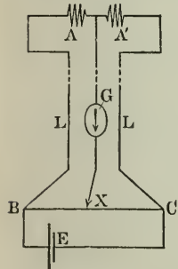
Thermophon.
