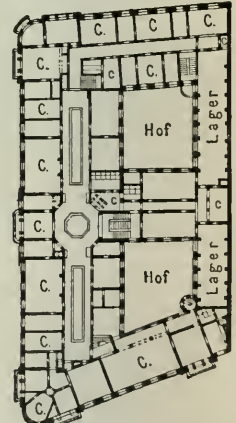
12. Dovenhof in Hamburg, I. Stock.
