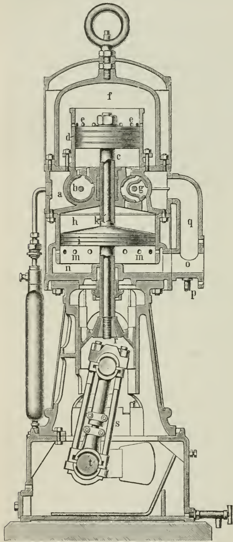
Fig. 1. Verbundmaschine, System Roworth.
