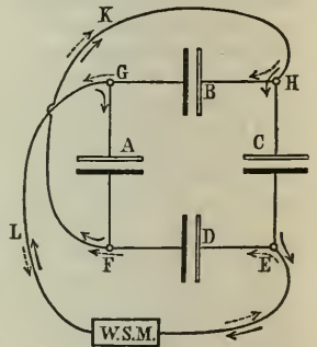
Pollacks Transformator.
