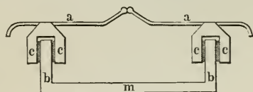
Spinthrometer.
