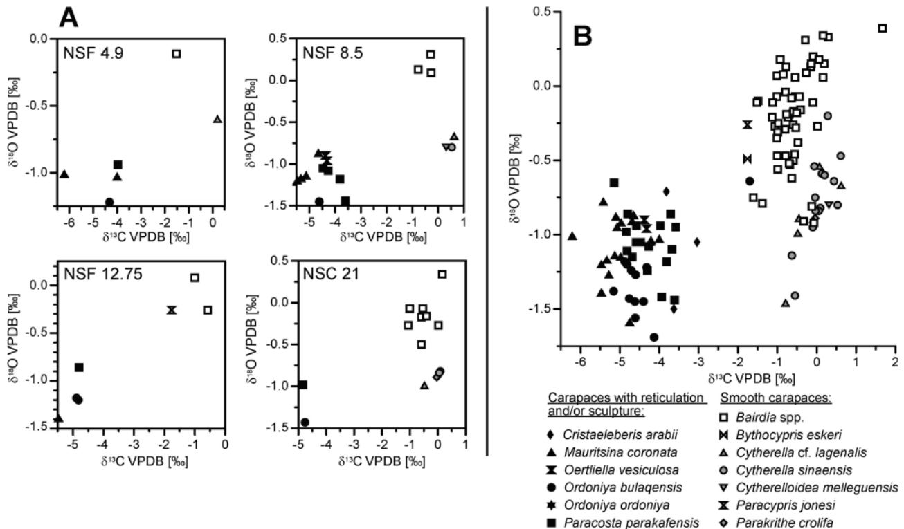
FIGURE 3: \delta^{13}\text{C} - \delta^{18}\text{O} cross plots of the Danian ostracode samples from Tunisia. (A) Selected samples, (B) all analyses from the NSF and NSC sections.
