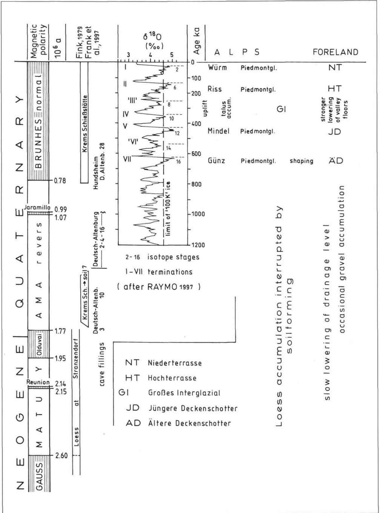
Fig. 1 Temporal position of geological activities in Austria during the Quaternary in comparison to the paleomagnetic and δ 18 O timescale.
