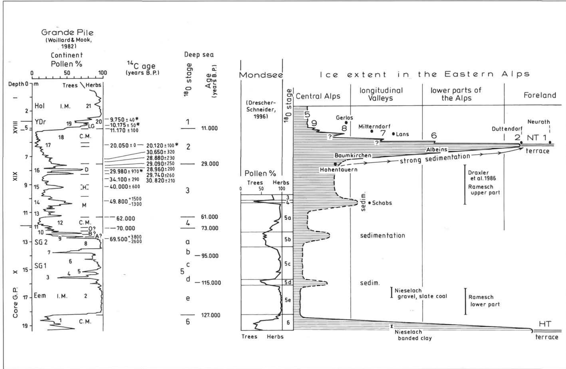
Fig. 11 Temporal development of the ice extent in the Eastern Alps, according to the sites described, and the sedimentation model (see Figs. 9, 10) compared to the pollen profiles from Mondsee and Grande Pile.
