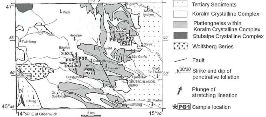
Fig. 2: Tectonic map of the Koralm area; the sampling sites and corresponding structural data are marked.
