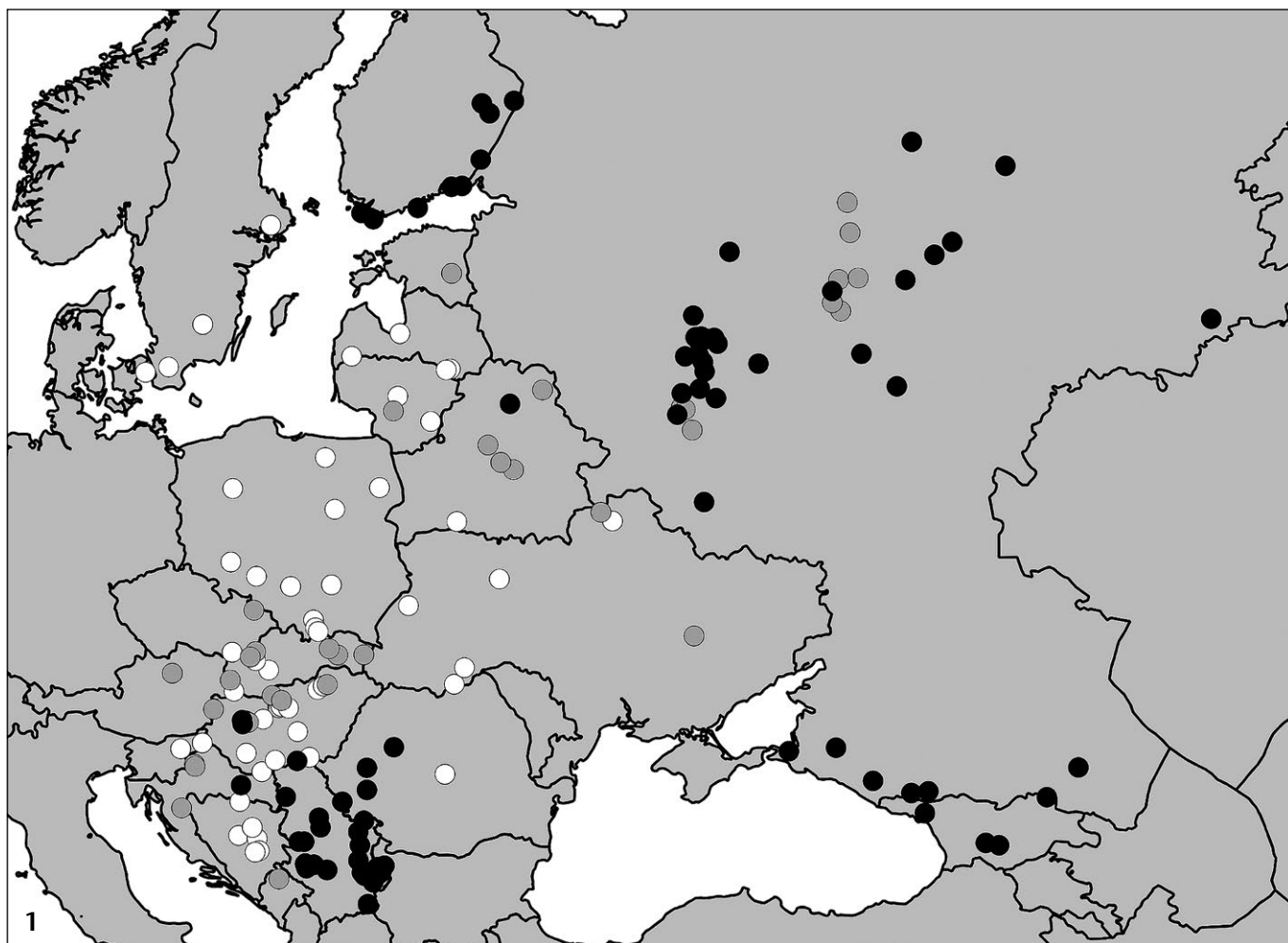
Fig. 1: Distribution of Nymphalis vaualbum in Europe. White dots represent records from 1900–1950; grey dots denote records from 1950–2000 and black dots represent records from 2000–2013. — Map prepared by MĐ.
