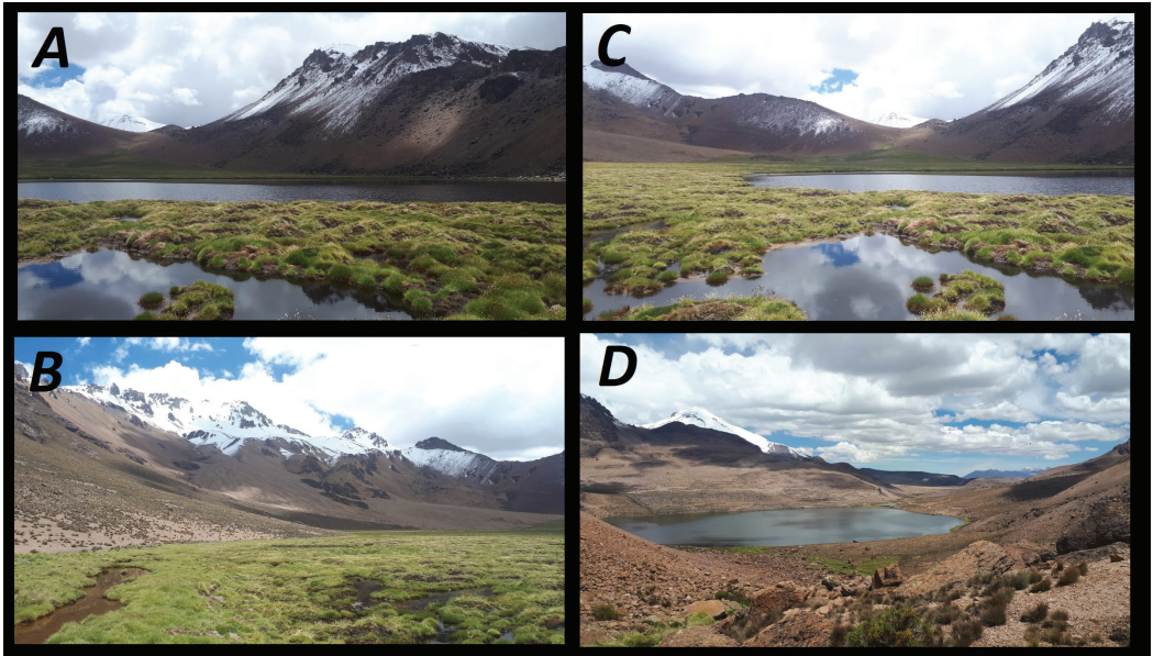
Figure 4. A–C. Northern Andean Lake Sora Pata, near Caquena village in the Chilean Altiplano and Bolivian border; D. View from Sora Pata to Casiri Macho Lake at 4838 m.
