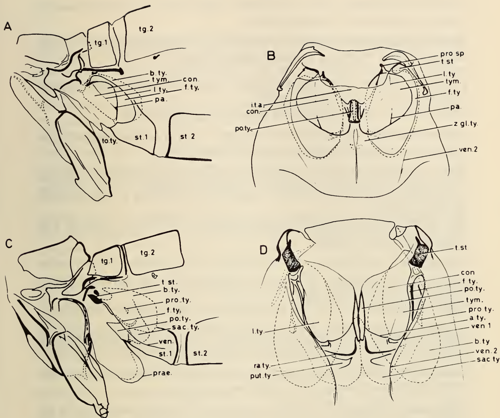
Pl. 2. Tympanal organs in Pyralidae.
