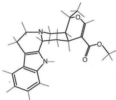
Akuammigine (6)
