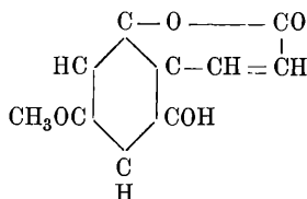
Methyldioxycumarine
