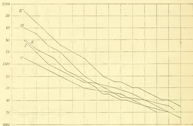
Fig. 8. Labrador-Nephelin (Mineralgemenge).
