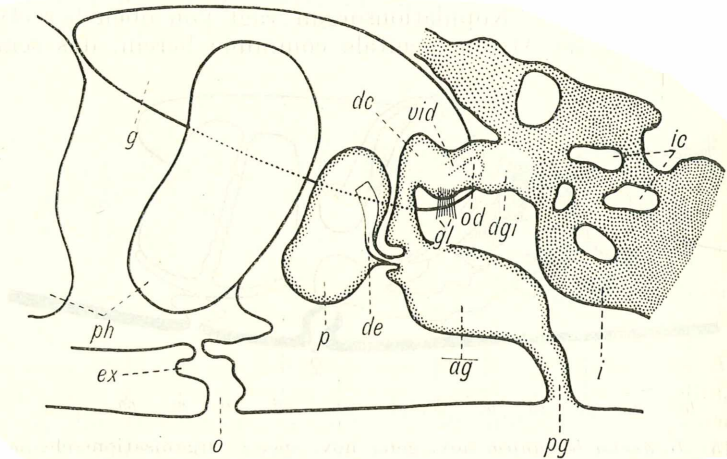
Fig. 16. Kambanella agilis Steinböck. Organisationsschema des Genitalapparates. ag = Atrium genitale; dc = Ductus communis; de = Ductus ejaculatorius; dgi = Ductus genito-intestinalis (Bursa seminalis); ex = Exkretionsbecher; g = Germar; gl = Schalendrüsen; i = Darm; ic = Darmvacuolen; o = Mundöffnung; od = Ovidukt; p = Kopulationsorgan; pg = Porus genitilis; ph = Pharynx; vid = Vitelloductus. (Aus Steinböck 1931.)
