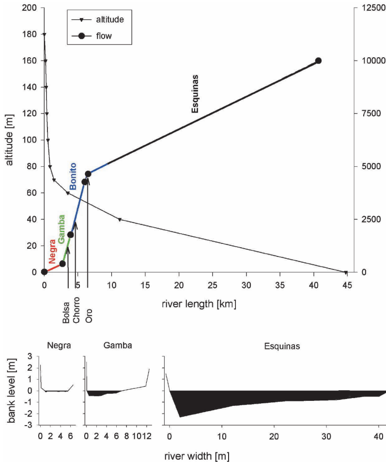
Fig. 2: River length [km] versus altitude [m] and flow [ l s^{-1} ] during the dry season 2004 of the Quebrada Negra flowing into Quebrada Gamba, Río Bonito and Río Esquinas. Tributaries like Quebrada Bolsa, Quebrada Chorro and Río Oro are indicated.
