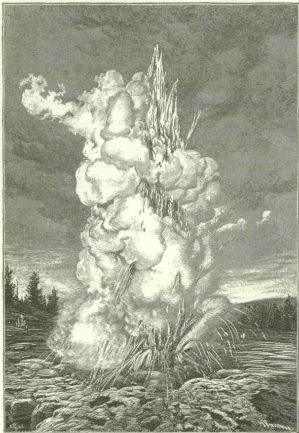
Grand-Geysir in Action (1878).
