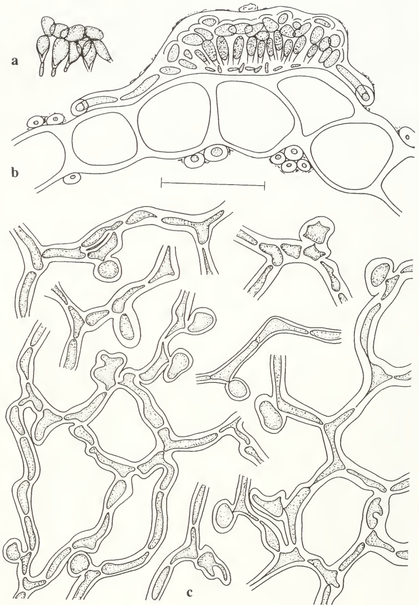
Fig. 2: Bryonectria callicarpa (M, holotype). a: Phialides; b: Section through dome-like structure of anamorphic state with phialides on leaf surface; c: Hyphae with appressoria. Scale bar: a-c: 20 µm.
