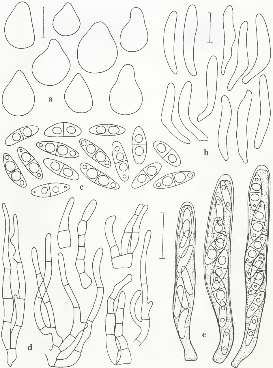
Fig. 1: Bryonectria callicarpa (M, holotype). a: Ascospores in outline; b: Asci in outline; c: Ascospores; d: Apical paraphyses; e: Immature (left) and mature asci. Scale bars: a: 100 \mu m; b: 25 \mu m; c-e: 15 \mu m.
