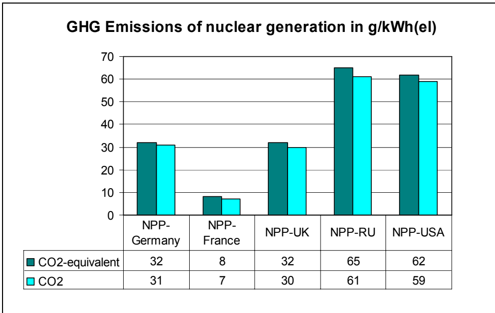
Figure 4: Greenhouse gas Emission of Nuclear Generation (FRITSCH 2007).
