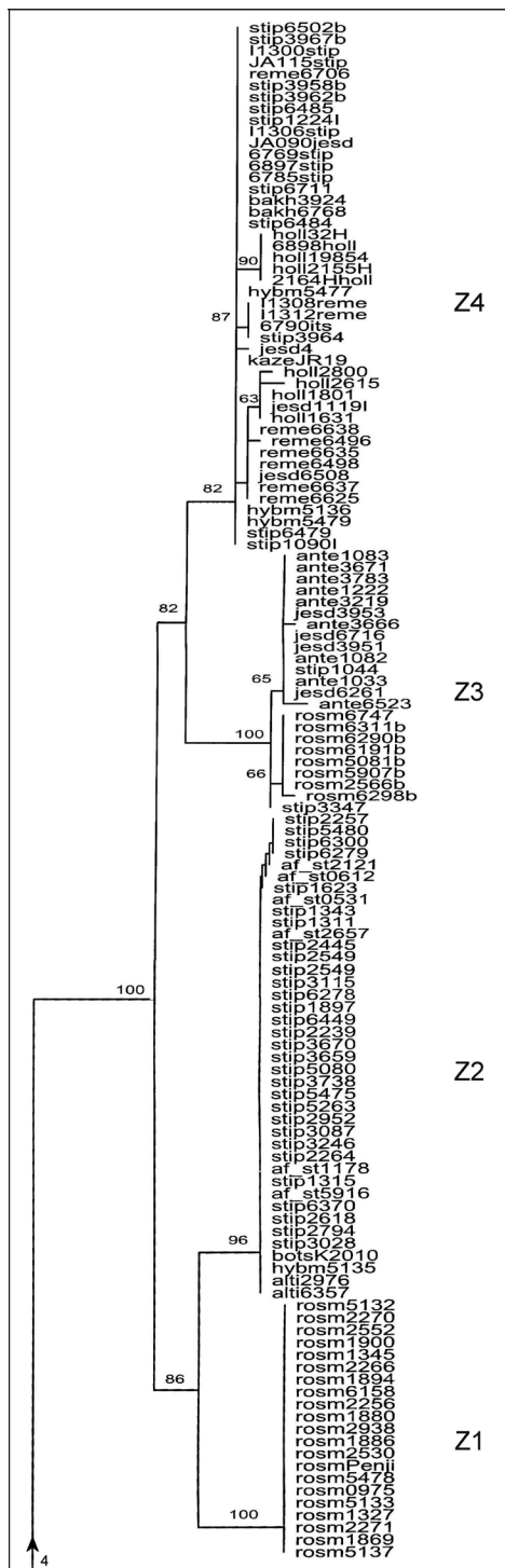
Fig. 6: Upper sector of a RAxML dendrogram based on ITS sequences of subgenus Melanocrommyum showing the most upper part of the core clade at positions Z1 - Z4. Arrowhead 4 marks the connection to the top of Fig. 5. - Abb. 6: Oberster Abschnitt eines RAxML-Dendrogramms der ITS-Sequenzen von subgenus Melanocrommyum , der die Clades an den Positionen Z1 - Z4 zeigt. Pfeil 4 markiert den Anschluss zur Spitze von Abb. 5.
