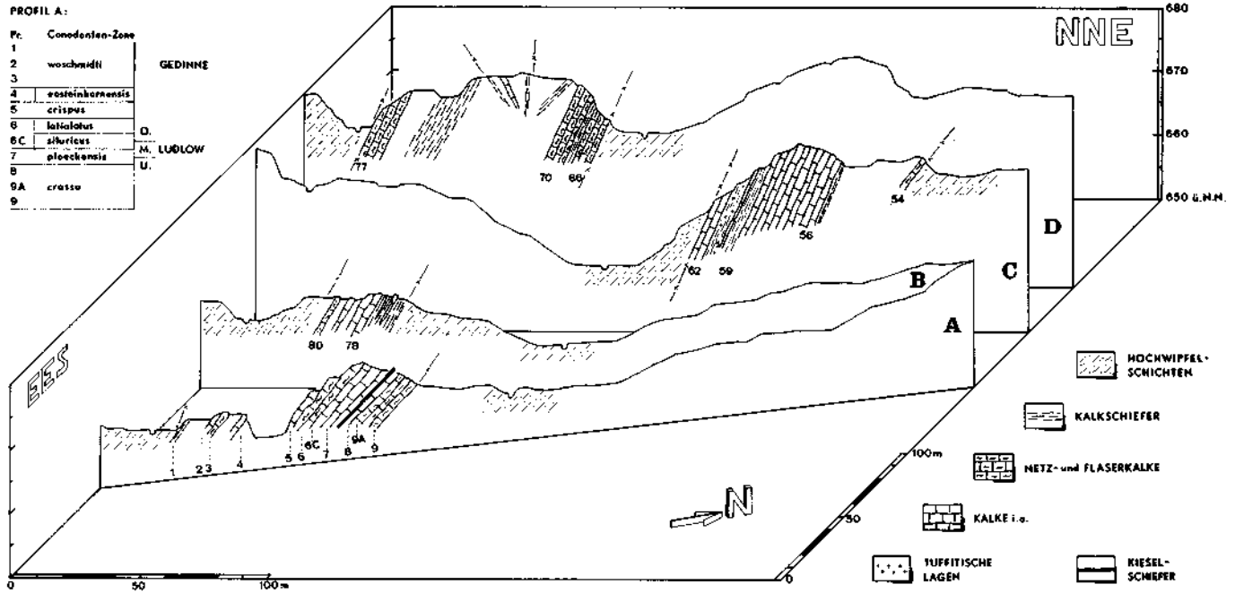
Abb. 2. Silur-Devon-Profile W Pessendellach.
