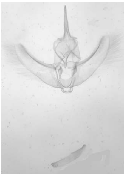
Abb. 8: Scodiomima crocallaria STAUDINGER, 1892, GU 1161 ♂ FW
