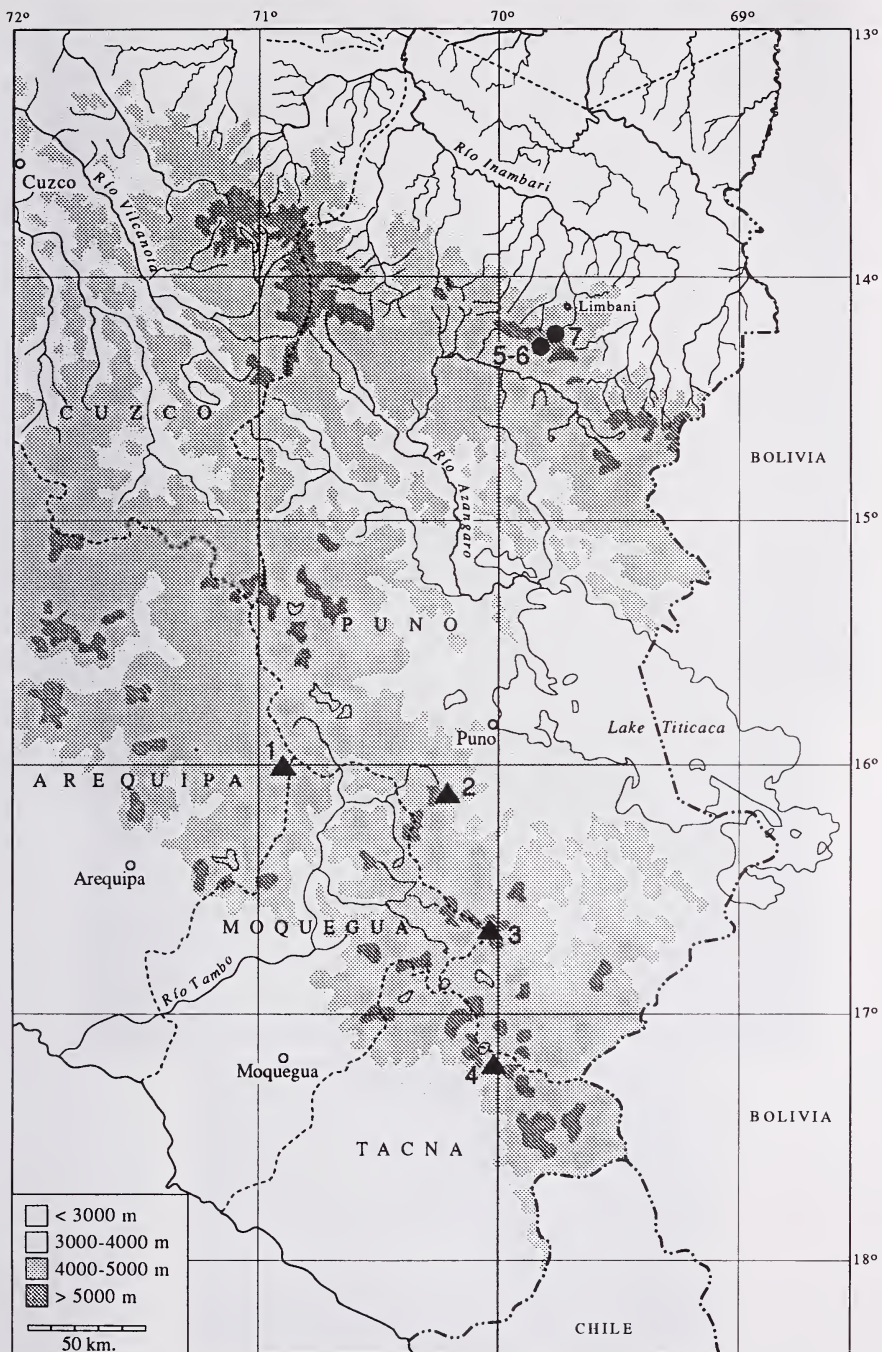
Fig. 1. Map of distribution of the puna mouse, Punomys , in southern Perú. Localities are numbered as in the Method and materials; localities 1–4 are of P. lemninus , 5–7 are of kofordi , new species.
