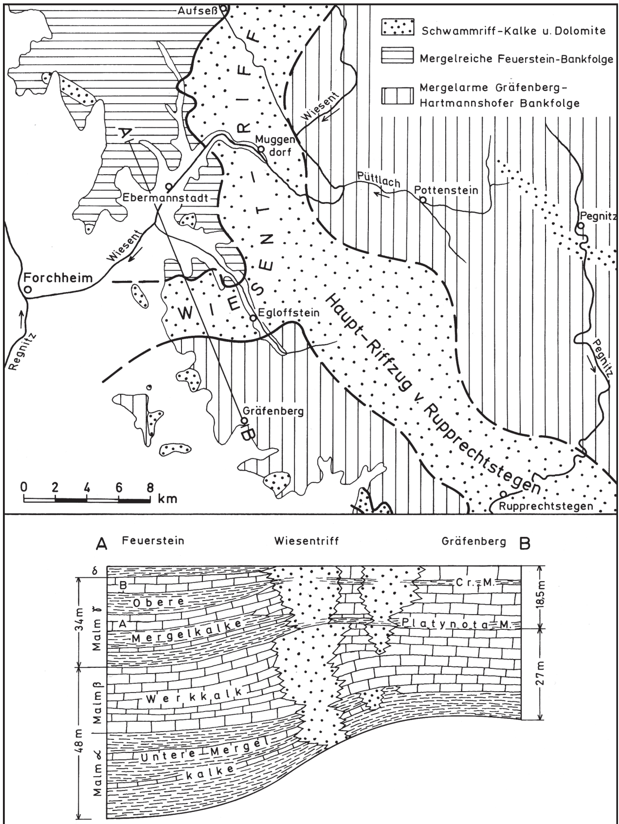
Figure 5: Cross section from west of the more marly Swabian Facies over the Wiesen-Reef Barrier into the more calcareous facies of the Northern Franconian Alb (after MEYER & SCHMIDT-KALER (1992)).
