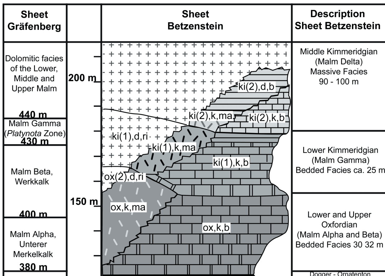
Figure 11: Comparison of the stratigraphic subdivisions and facies types documented in the geological sheet 6333 Gräfenberg (DORN 1958) and sheet 6334 Betzenstein (GOETZE et al. 1975). ox,k,b = bedded limestones and marls of the Oxfordian (Malm Alpha and Beta), ox,k,ma = sponge limestones of the Oxfordian, ox(2)d,ri = reef dolomite of the Oxfordian, ki(1),k,b = bedded limestones of the Lower Kimmeridgian (Malm Gamma), ki(1),k,ma = sponge limestones of the Lower Kimmeridgian, ki(1),d,ri = reef dolomite of the Lower Kimmeridgian, ki(2),k,b = bedded limestones of the Middle Kimmeridgian (Malm Delta), ki(2),k,ma = sponge limestones of the Middle Kimmeridgian, ki(2),d,b = thick-bedded dolomite (Tafelbankiger Dolomit) of the Middle Kimmeridgian, ki(2),d,ri = reef dolomite of the Middle Kimmeridgian.
