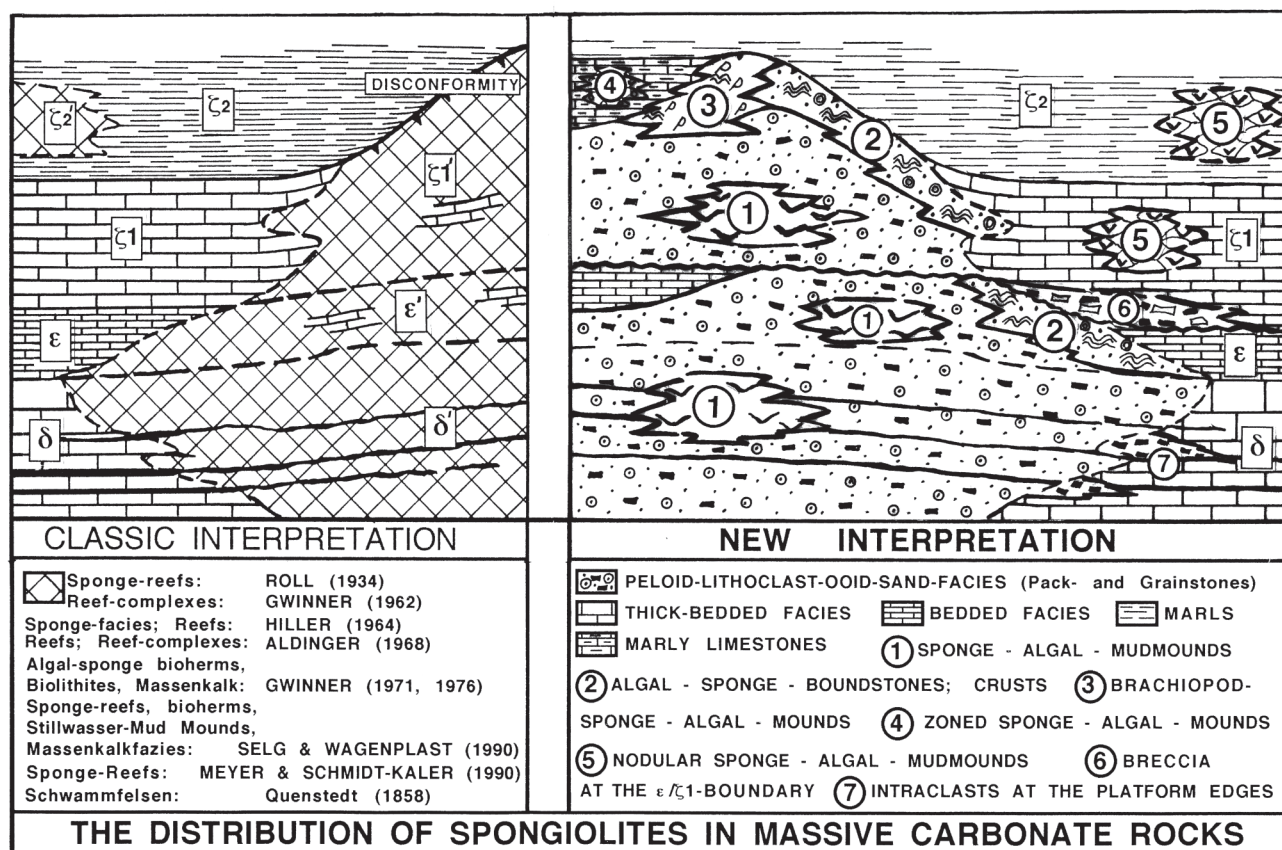
Figure 7: The distribution of spongiolites in massive carbonate rocks (“reef-complexes”, Massenkalk etc.). Comparison of the classic interpretation and the new interpretation. Note that the peloid-lithoclast-oid sand facies makes up the greatest amount of the “Massenkalk”. The spatial distribution of real algal-sponge-buildups in and around the carbonate sand facies is interpreted to be caused by varying hydrodynamic conditions triggered by the paleogeographic distribution of the carbonate sand facies. The Malm Epsilon/Zeta 1 boundary-breccia marks a regressive maximum. The rapid growth of brachiopod-algal-sponge-mounds in the Malm Zeta is caused by a transgressive trend beginning at the Malm Epsilon/Zeta 1 boundary (from KOCH et al. 1994).
