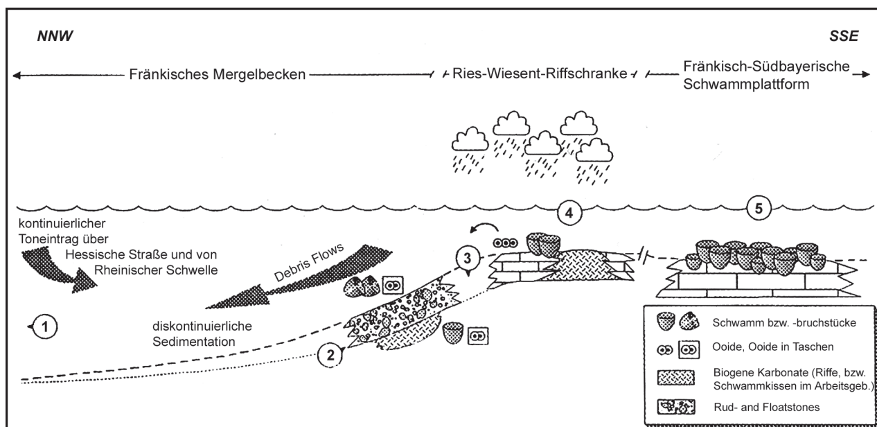
Figure 10: Sedimentation model for the Kimmeridgian 1 and 2 on the gentle dipping slope from the carbonate platform to the basin of Ebermannstadt at the outcrop of the Schießfels near Hardt. 1 = basin of Ebermannstadt, 2 = position of the Schießfels, 3 = thick-bedded platform limestones of Gräfenberg, 4 = ooid sands and sponge-algal crust facies on swells, 5 = facies of the Treuchtlingen Limestones in the Southern Alb (distance and relief not to scale; from TARASCONI 1996).
