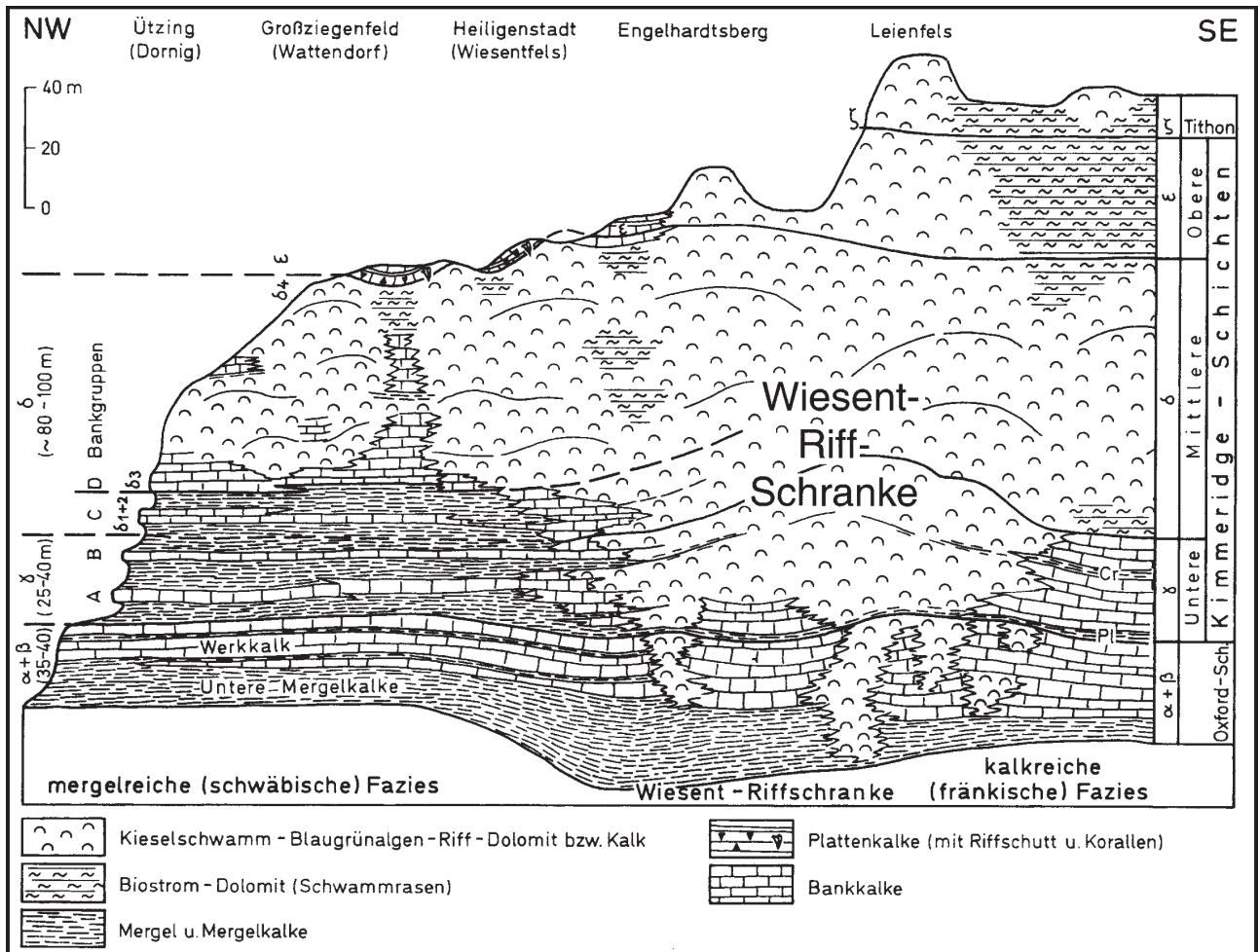
Figure 4: Facies scheme of the Northern Franconian Alb (after MEYER & SCHMIDT-KALER 1992 and MÄUSER et al. 2002) used in the last 40 years. The Wiesent-Reef barrier separates the sea floor in a more marly area (NW; Swabian Facies) and a carbonate platform in the SE (Franconian Facies). This reef barrier is especially effective in the Malm Alpha and Gamma/Lower Delta. Sponge reefs intensively develop during the Upper Malm Delta forming a reef platform expanded nearly over the complete area.
