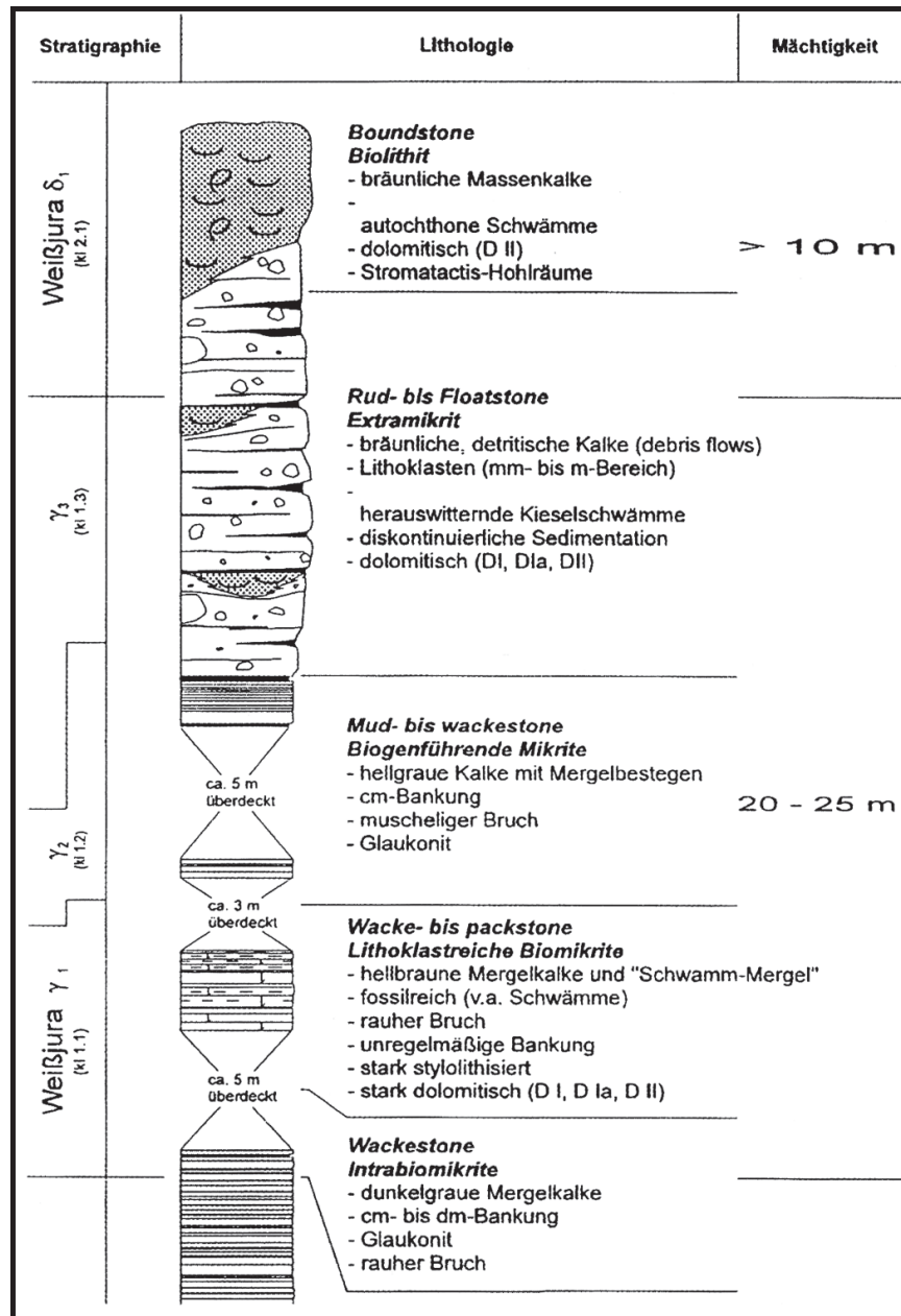
Figure 9: The profile up to the Schießfels near Hardt which marks the beginning of the growth of sponge-algal buildups in the uppermost Malm gamma (from TARASCONI 1996).
