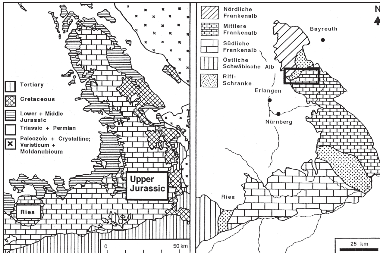
Figure 3a + b: (a) Simplified geological map of the pre-Quaternary sediments of the Franconian Alb and adjacent areas (after ZEISS 1977). (b) Main facies areas of the Upper Jurassic of the Franconian Alb. The area of the excursion is indicated in the rectangle.
