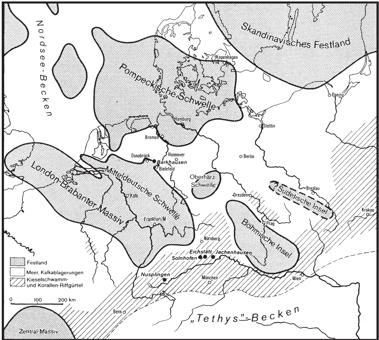
Figure 1: Distribution of land and sea in the Upper Jurassic and the position of the shallow epicontinental sea north of the Tethys (from MEYER & SCHMIDT-KALER 1992) indicating the distribution of siliceous sponges and corals.
