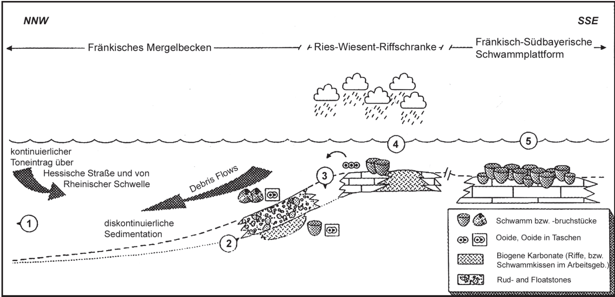
Figure 10: Sedimentation model for the Kimmeridgian 1 and 2 on the gentle dipping slope from the carbonate platform to the basin of Ebermannstadt at the outcrop of the Schießfels near Hardt. 1 = basin of Ebermannstadt, 2 = position of the Schießfels, 3 = thick-bedded platform limestones of Gräfenberg, 4 = ooid sands and sponge-algal crust facies on swells, 5 = facies of the Treuchtlingen Limestones in the Southern Alb (distance and relief not to scale; from TARASCONI 1996).
