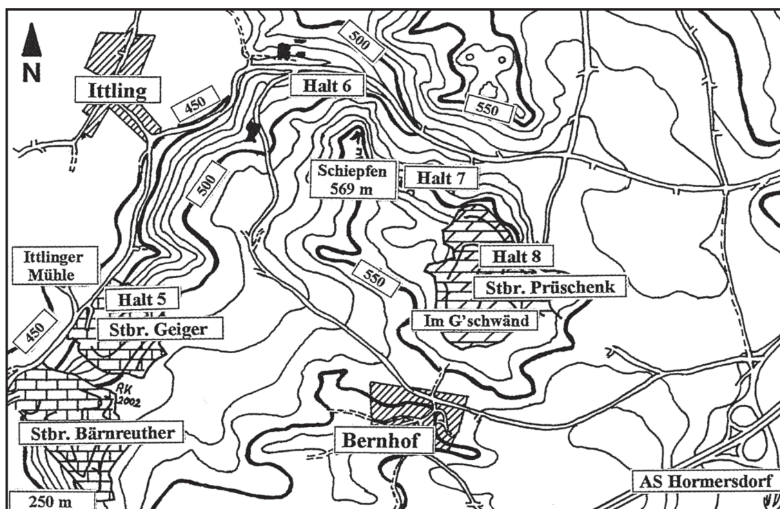
Figure 12: Detail map showing the eastern area of the excursion with the quarries of the Geiger and the Prüschenk companies as well the stops (Halt) 5, 6, 7, and 8 in stratigraphic order (from KOCH et al. 2003).
