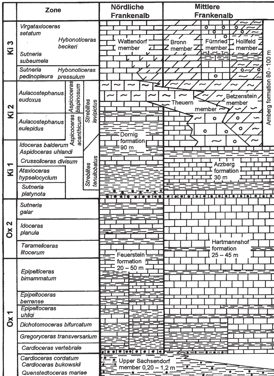
Figure 6: Biostratigraphic subdivision of the Oxfordian and Kimmeridgian, important ammonites, and facies differentiation in the Northern and Middle Franconian Alb (ZEISS 1966). The subdivisions of the lithologic columns in the Oxfordian indicate the different facies developments in the northern and southern part of the Northern Franconian Alb and of the western and eastern areas in the Middle Franconian Alb.
