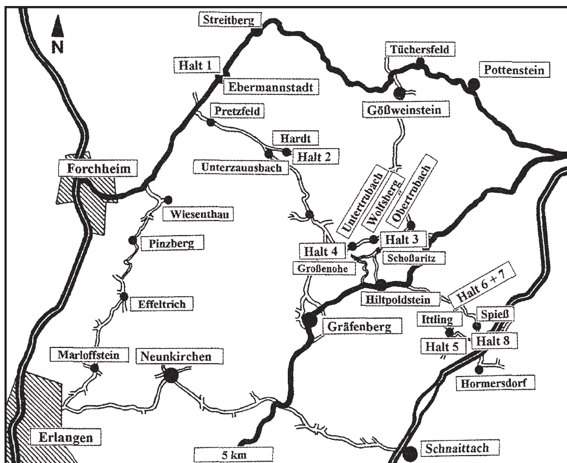
Figure 8: The excursion route including stops (Halt) 1-8 in the Northern Franconian Alb.
